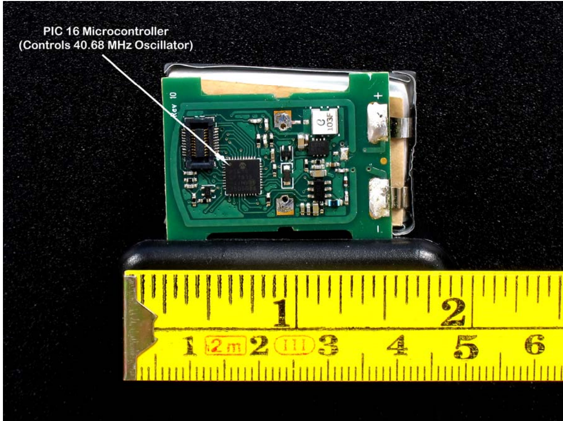
Control Board – Front side
