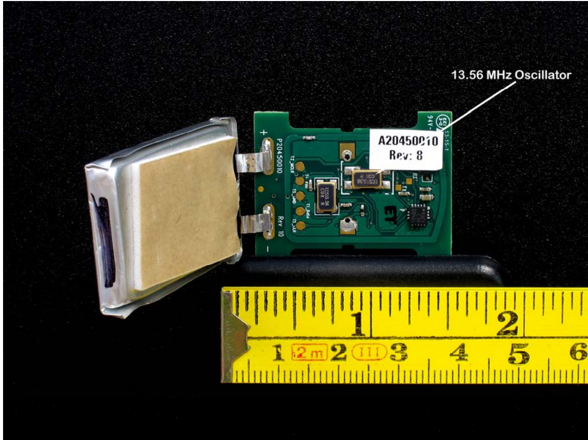
Control Board – Back Side
