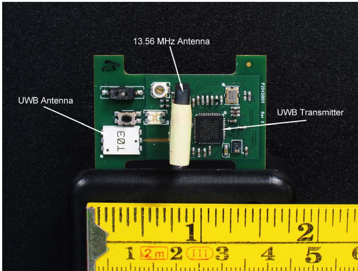
UWB Board – Front Side
