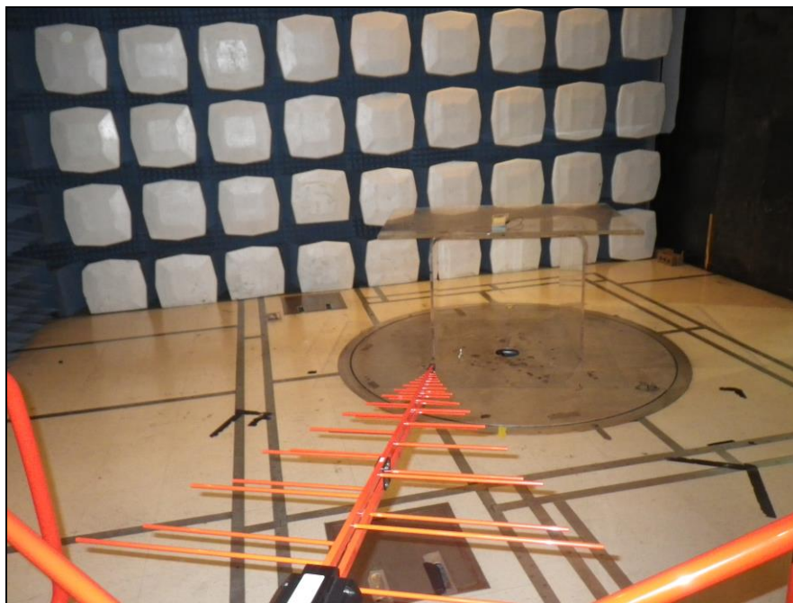
Photograph 3. Fundamental Field Strength & Harmonic Emission, Test Setup
