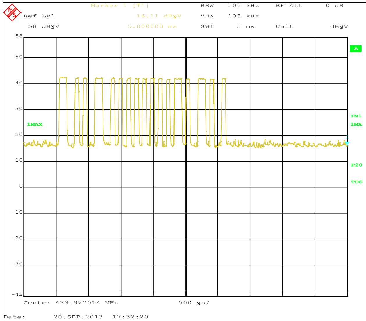
Figure 1 – Transmitter ON Time
