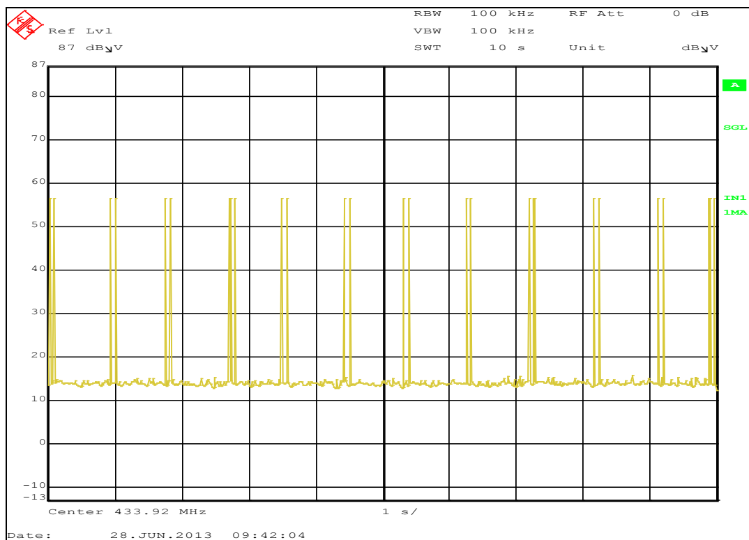
Plot 3. Duty Cycle, Period (Pattern Repeats Every 1s)
