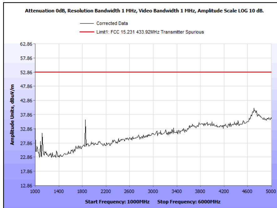
Plot 6. Radiated Spurious Emissions, 1 GHz – 5 GHz
