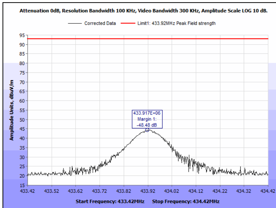
Plot 4. Fundamental Radiated Emissions, 433.92 MHz, Peak
