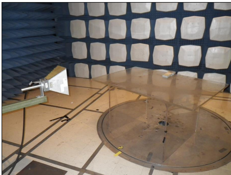
Photograph 5. Radiated Spurious Emissions, Test Setup, 1 GHz – 5 GHz
