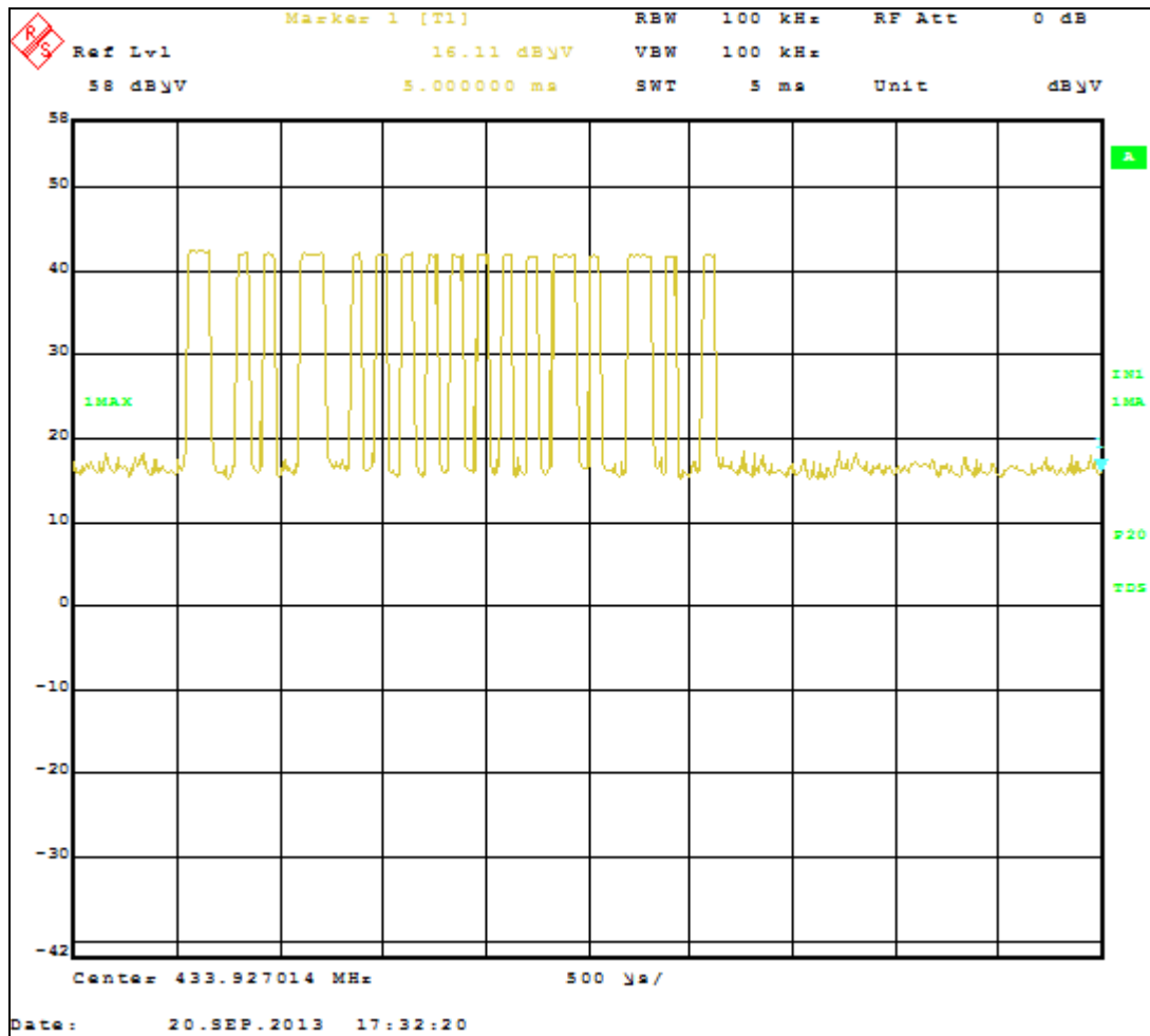
Plot 2. Duty Cycle, Transmitter ON Time
