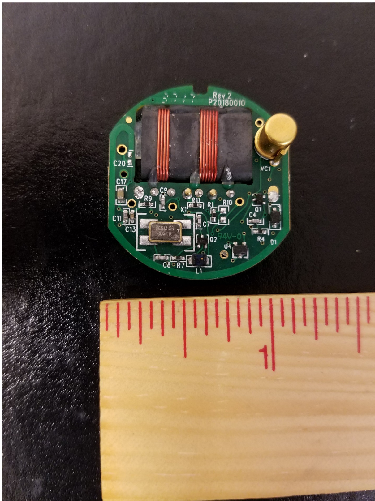
Internal bottom
