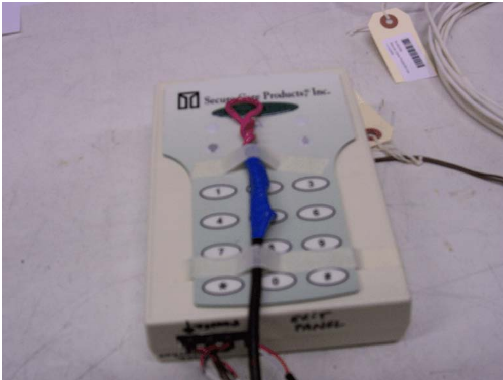
CONDUCTED EMISSIONS SETUP PHOTOGRAPH
