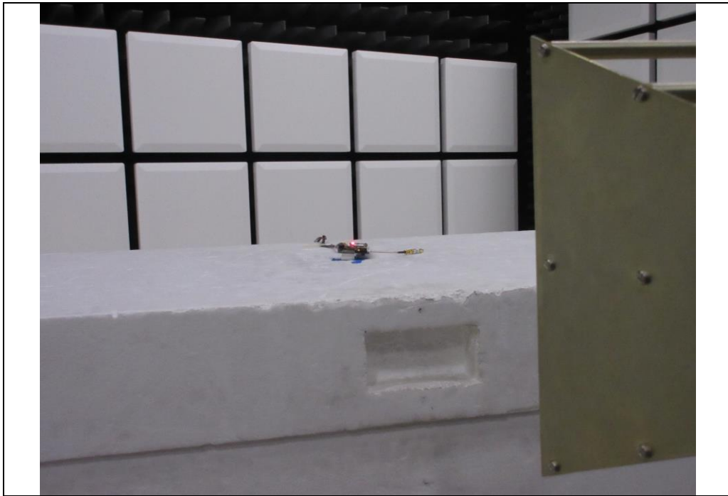
RF Radiated #4
