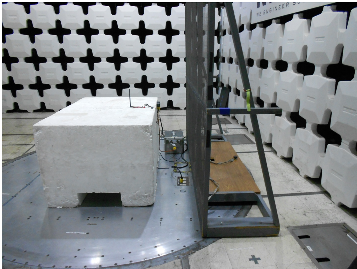
AC Power Conducted Emissions Test Configuration Photographs
