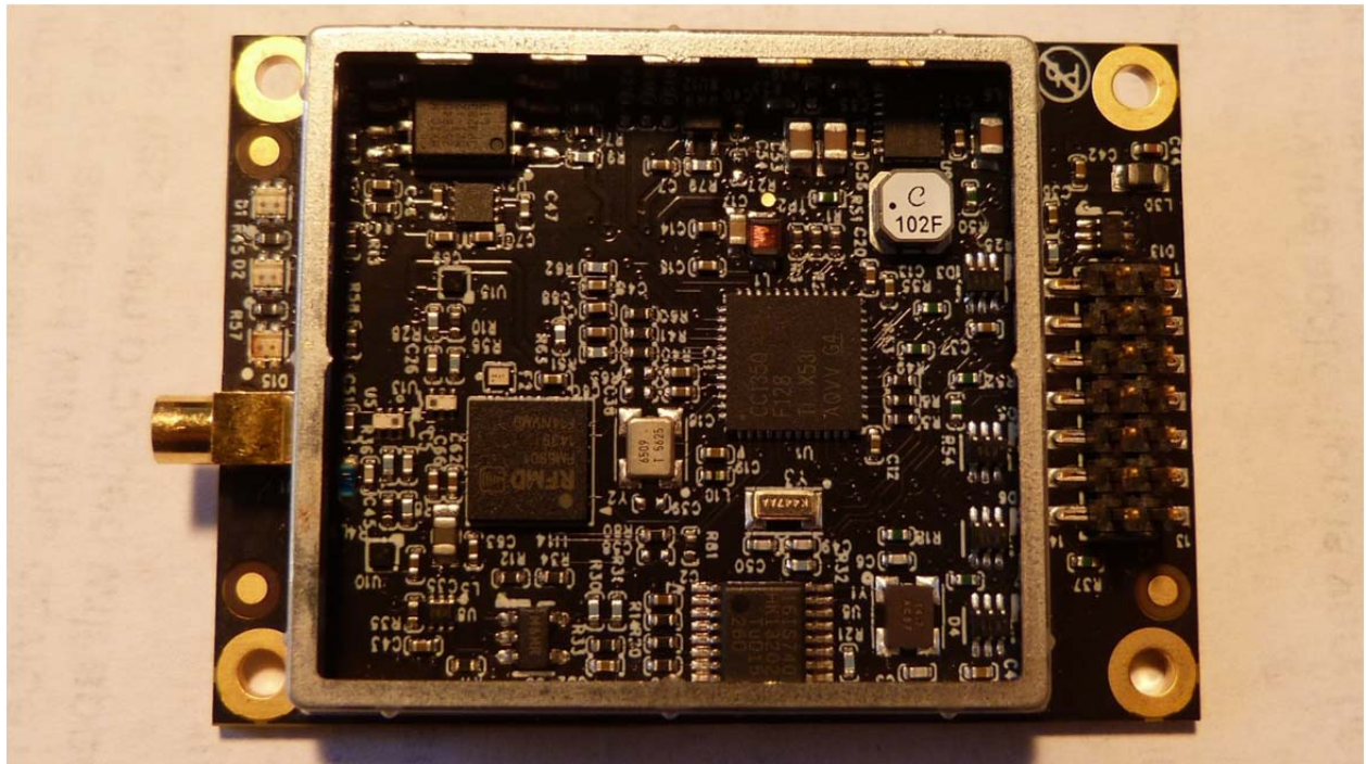
Z9-T Top w/o shield
