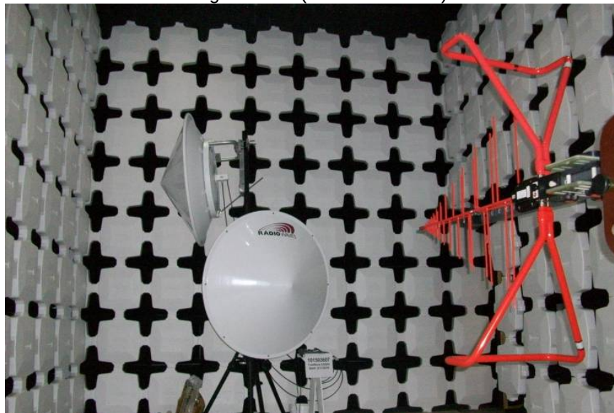
Bilog Antenna (30MHz to 1GHz)
