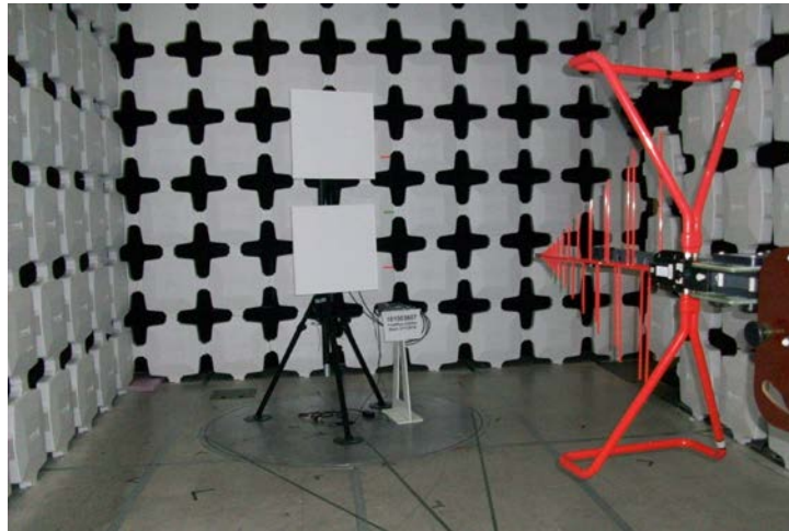
Bilog Antenna (30MHz to 1GHz)
