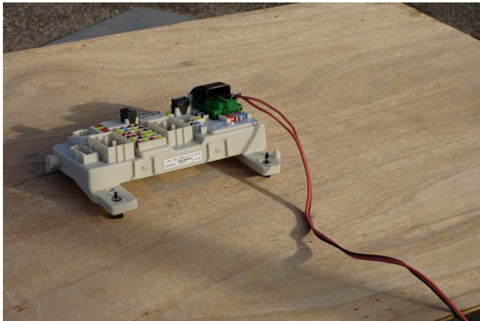
DUT on OATS (close-up)
