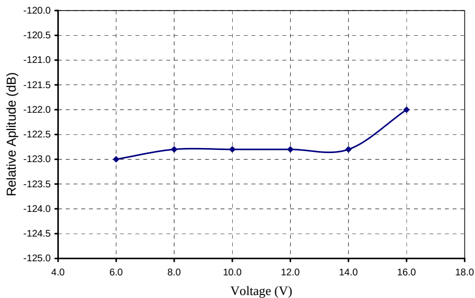
Figure 6.2. Relative emission at vs. supply voltage.
