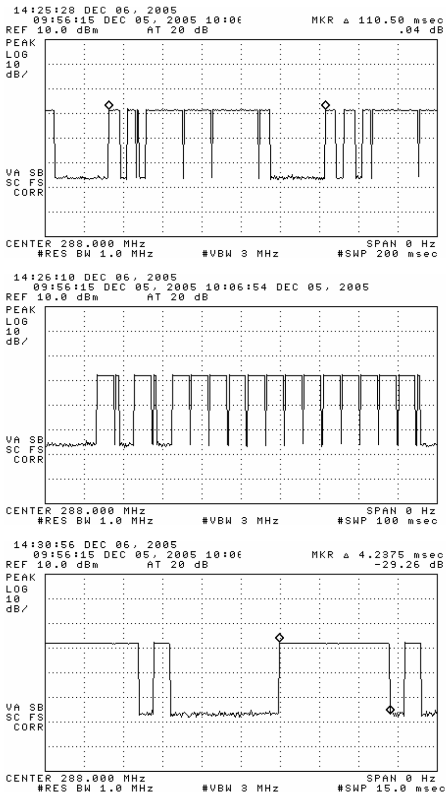
Figure 6.1(e). Transmissions modulation characteristics, 288 MHz: (top) low duty complete transmission, (center) expanded bit, (bottom) expanded period.
