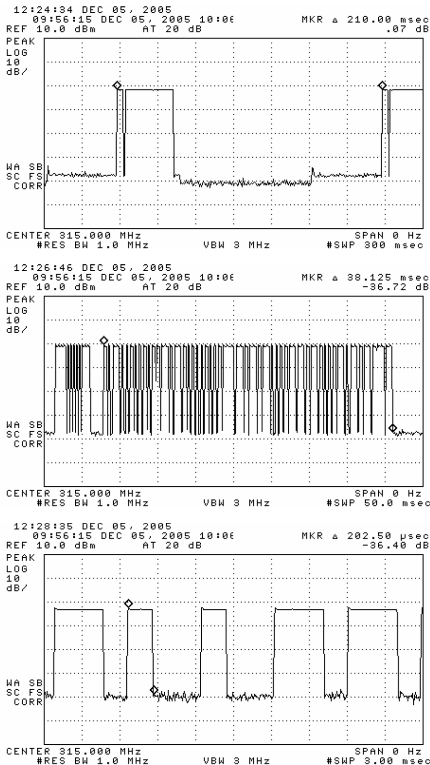
Figure 6.1(d). Transmissions modulation characteristics, 315 MHz: (top) high duty complete transmission, (center) expanded bit, (bottom) expanded period.
