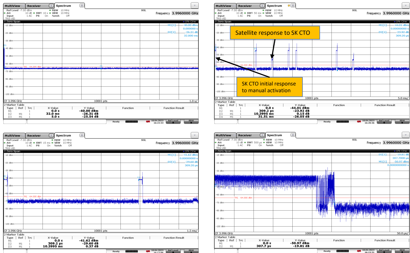
Figure 5: Fundamental Emission Pulsed Operation.
