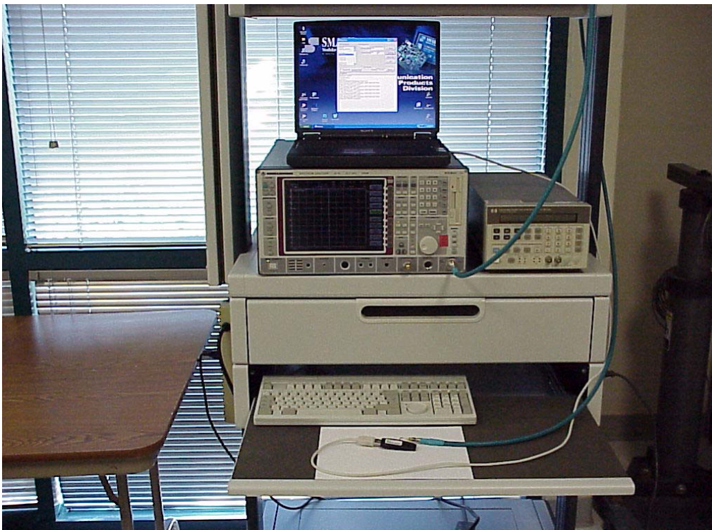
Test Setup
