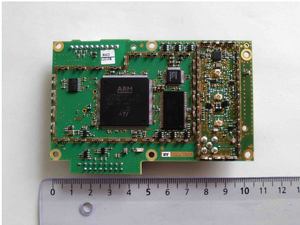
Main board (bottom view ), without shielding
