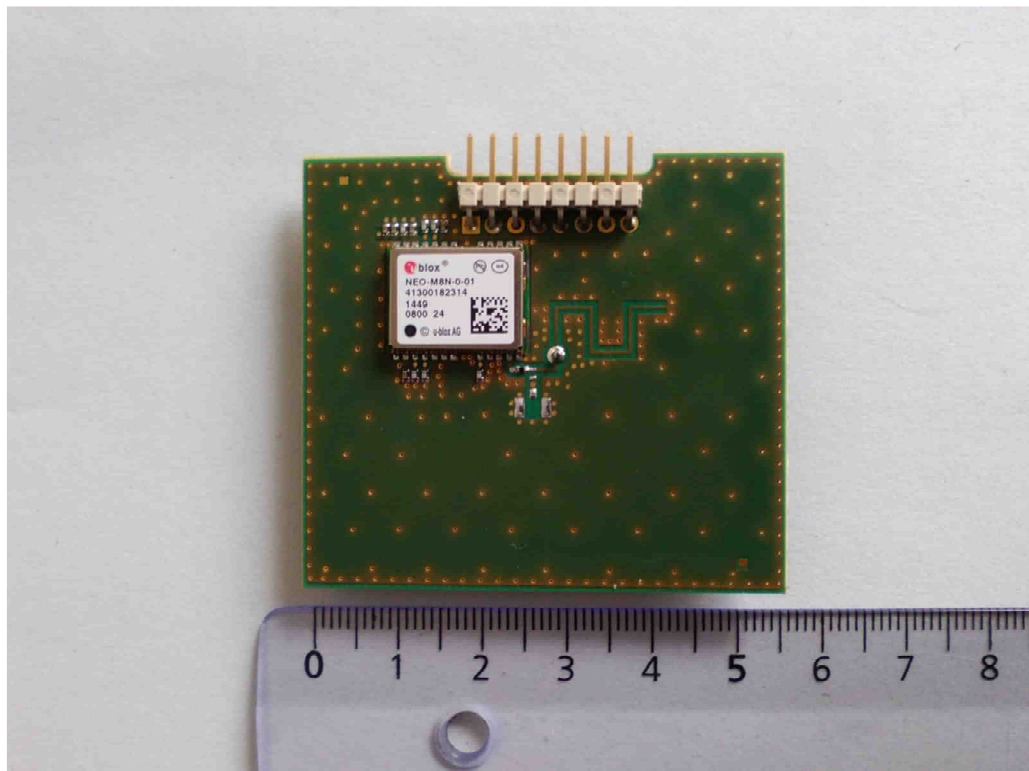
GPS board (bottom view)
