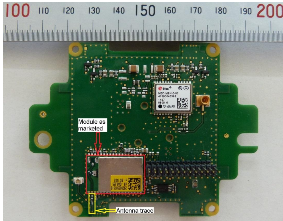
145298_29.JPG: Reference Design with EUT– Top View
