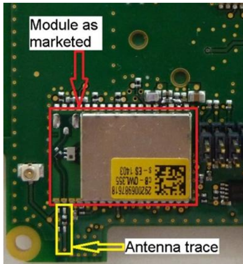
145298_30.JPG: Reference Design with EUT– Detail Top View
