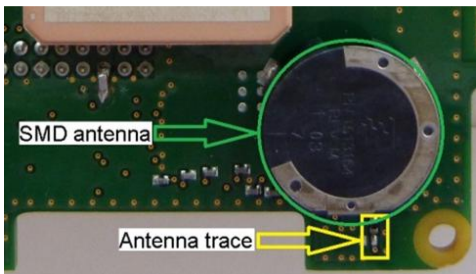
145298_34.JPG: Reference Design with EUT– Detail Bottom View
