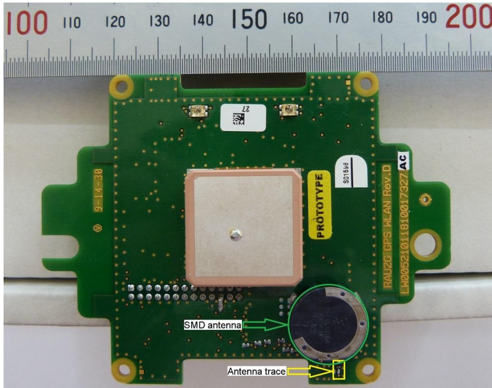
145298_33.JPG: Reference Design with EUT– Bottom View
