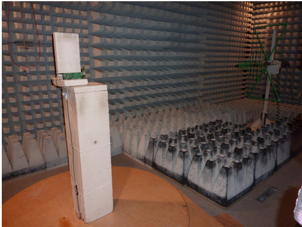
145298_18.jpg: Test setup - Radiated emission (fully anechoic chamber)
