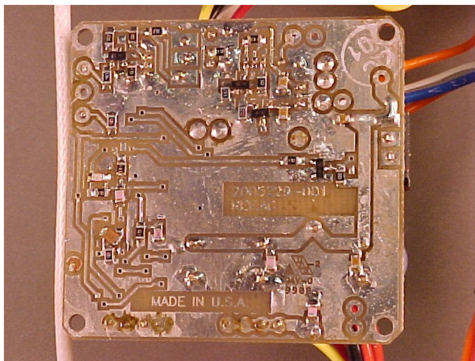
Photo 14. Transmit Power Control, bottom view.
