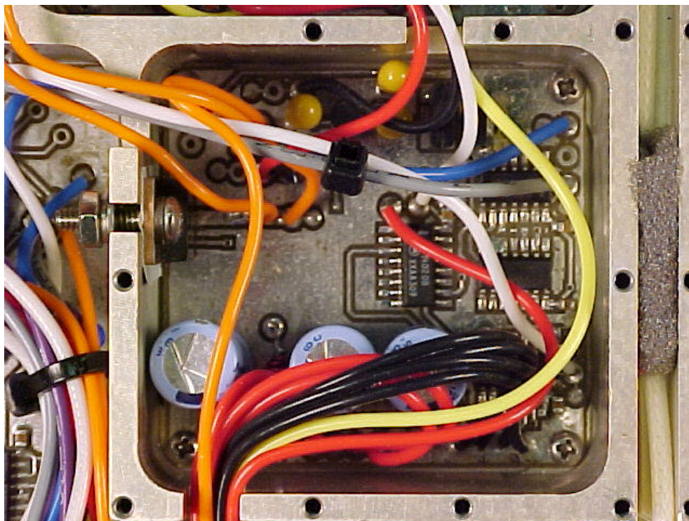
Photo 13. Transmit Power Control, top view.
