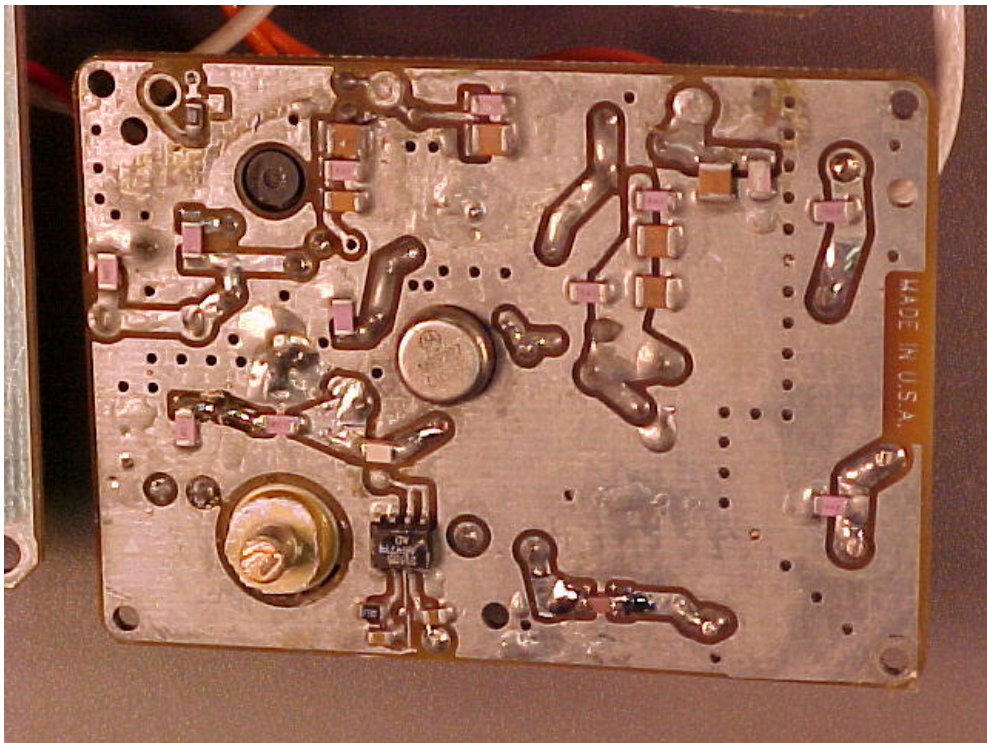
Photo 12. Transmit Power Amp, bottom view.
