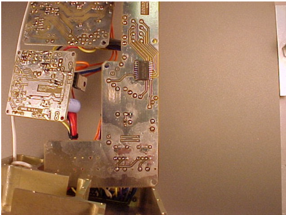
Photo 10. Transmit Interface, bottom view.
