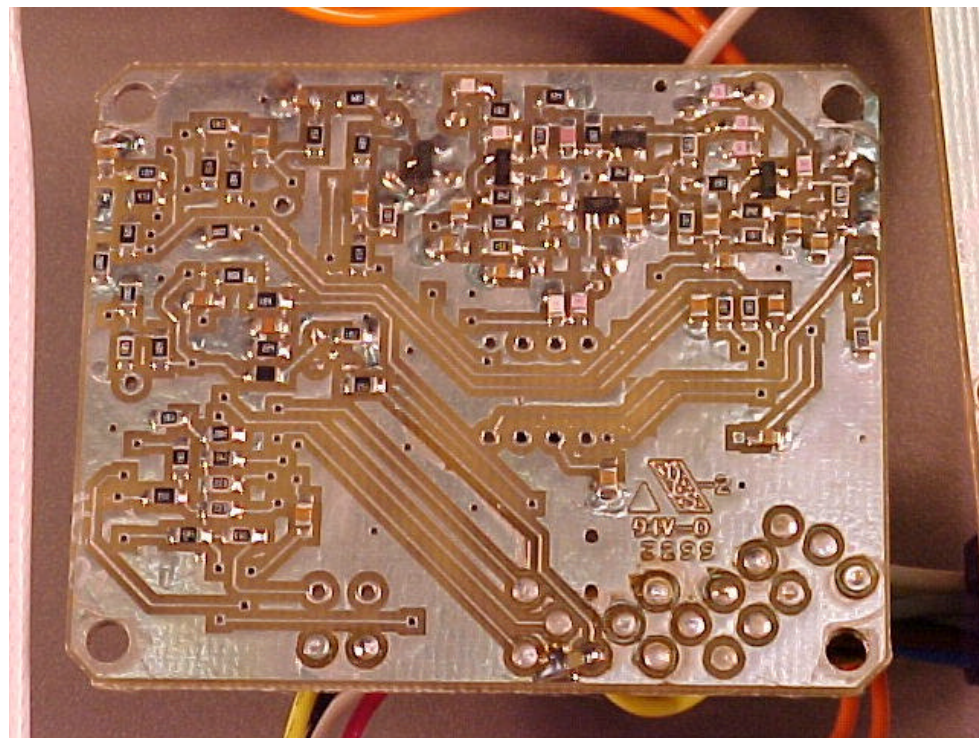
Photo 16. Transmit Synthesizer, bottom view.
