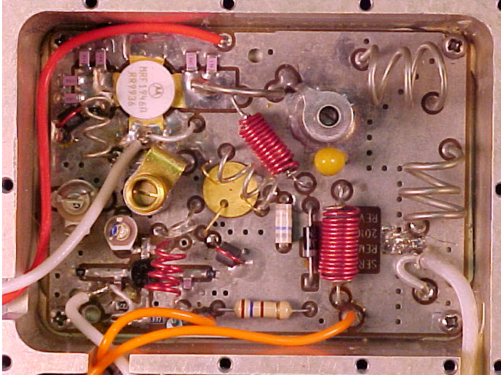
Photo 11. Transmit Power Amp, top view.
