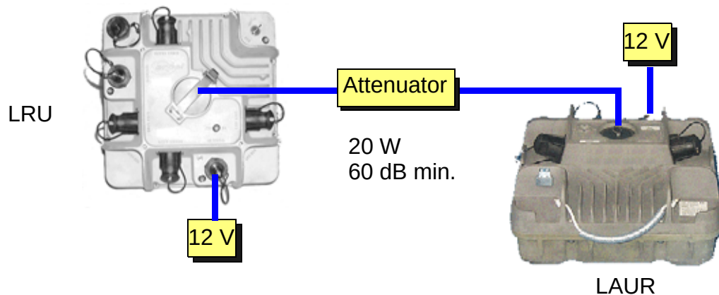
Figure 2 Test setup
