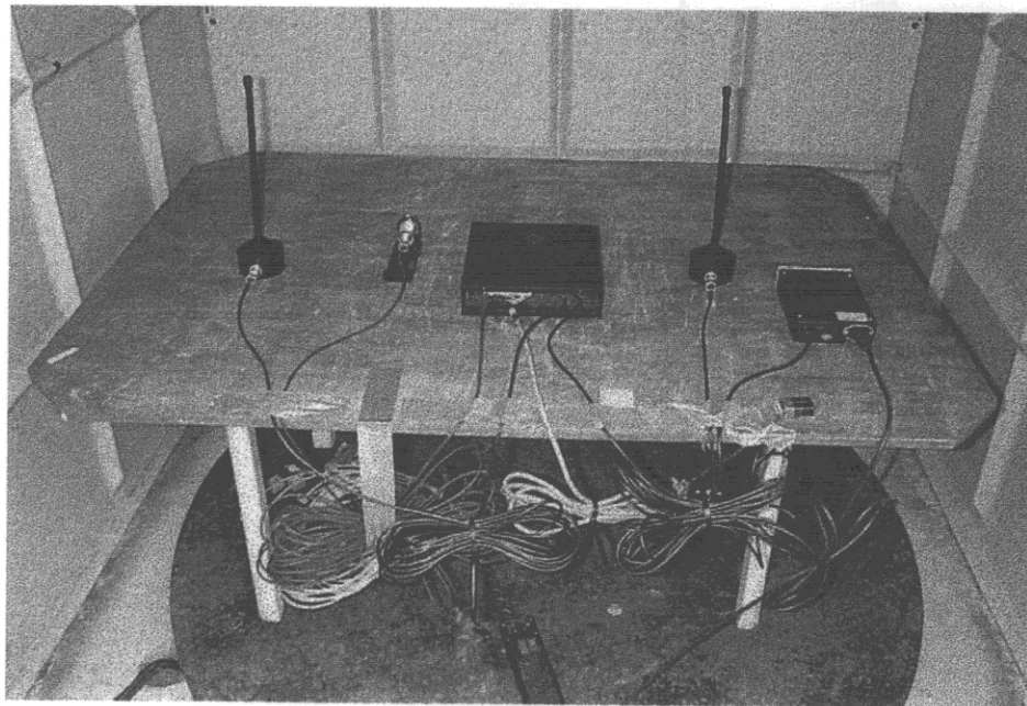
Photograph A-1 Title: Test site with Rx, radiated & conducted.
