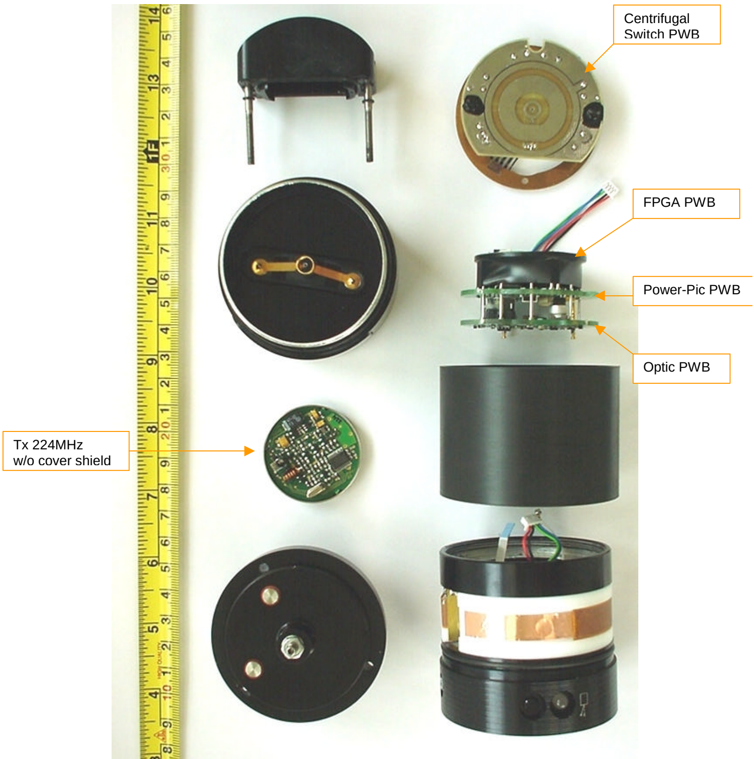
Title : Disassembled unit parts.
