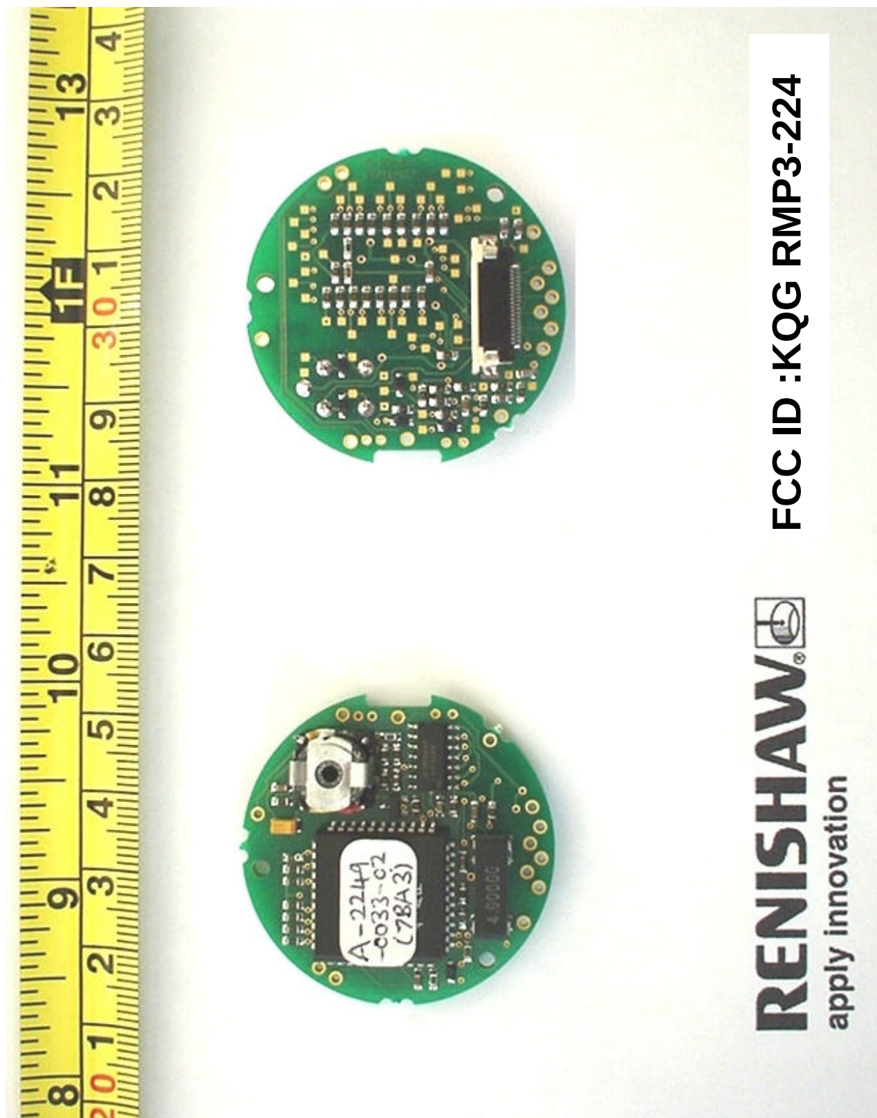
Title : Fpga PWB, top and bottom.
