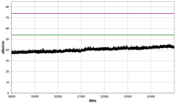
18 GHz to 25 GHz
