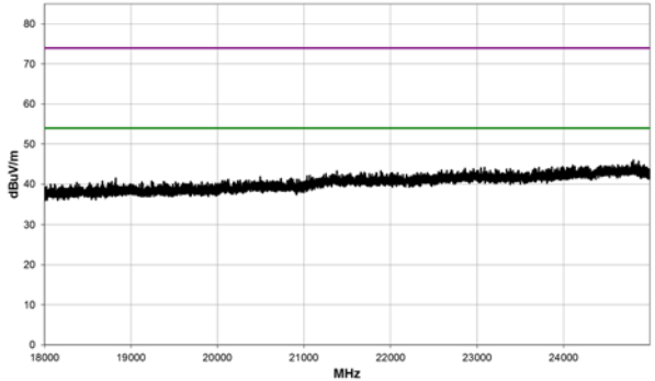
18 GHz to 25 GHz
