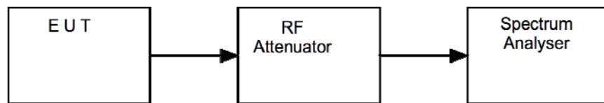
Figure iv Test Setup
