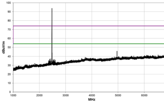
1 GHz to 7 GHz
