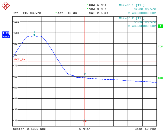
2480 MHz Upper Band Edge Plot – Peak
