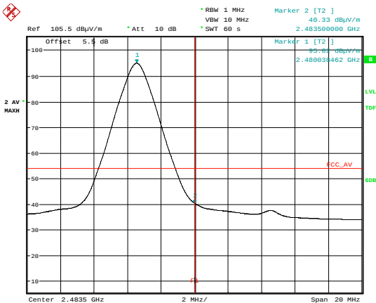
2480 MHz Upper Band Edge Plot - Average
