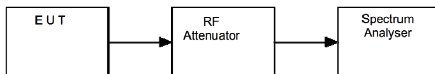
Figure vi Test Setup
