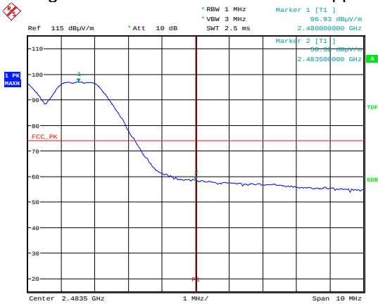
2480 MHz Upper Band Edge Plot – Peak
