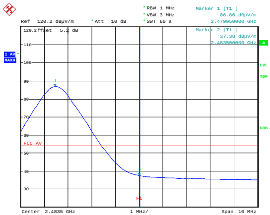
2480 MHz Upper Band Edge Plot - Average
