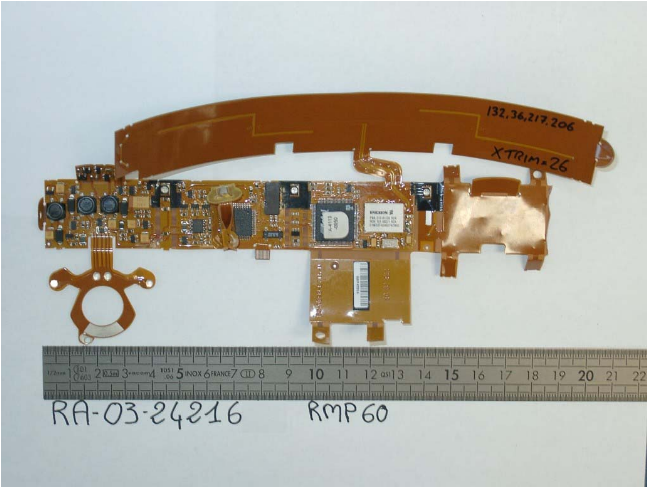
Printed circuit board transmitter: face 1
