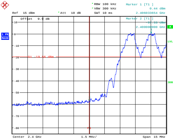
Lower band edge hopping channel
