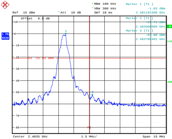
Upper band edge single hopping channel
