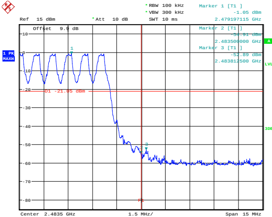
Upper band edge hopping channel
