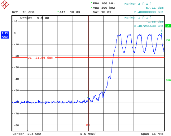
Lower band edge hopping channel
