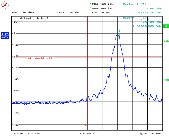
Lower band edge single hopping channel
