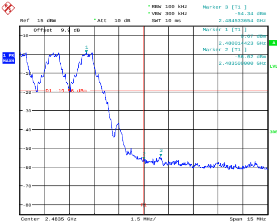
Upper band edge hopping channel
