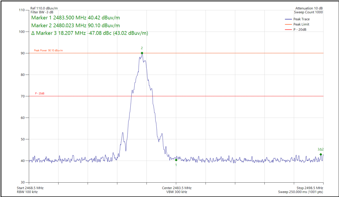
Figure 9 - CH39_BLE2M_ABE, 2480 MHz, Band Edge Frequency 2483.5 MHz
