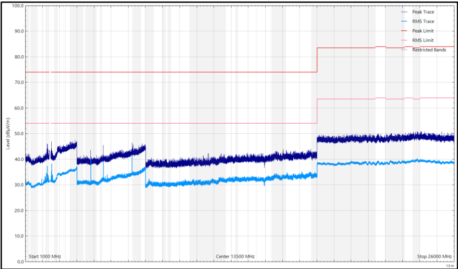
Figure 27 - CH37_LE2M_Y, 2404 MHz, 1 GHz to 26 GHz, Vertical
