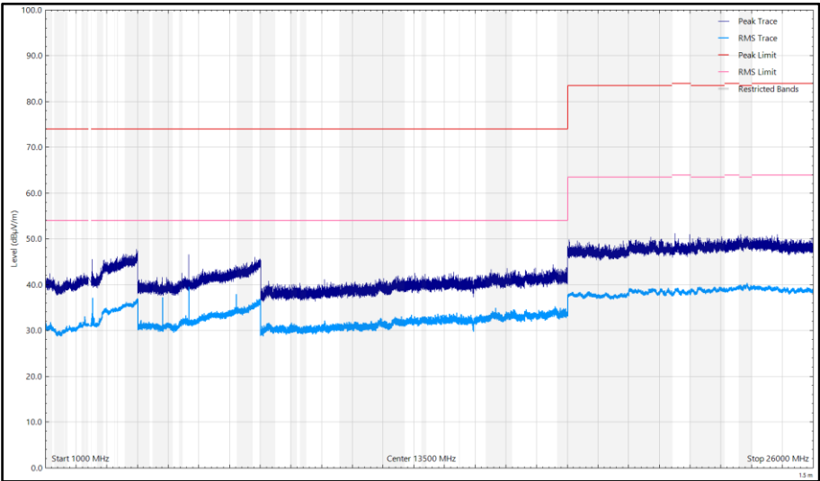
Figure 23 - CH37_LE2M_X, 2404 MHz, 1 GHz to 26 GHz, Vertical
