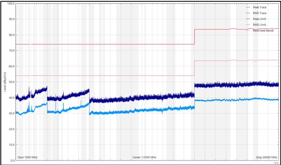
Figure 31 - CH37_LE2M_Z, 2404 MHz, 1 GHz to 26 GHz, Vertical
