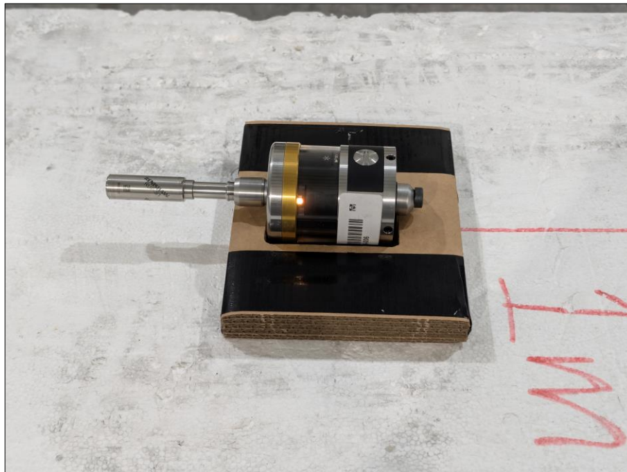
Figure 60 - Test Setup – X Orientation
