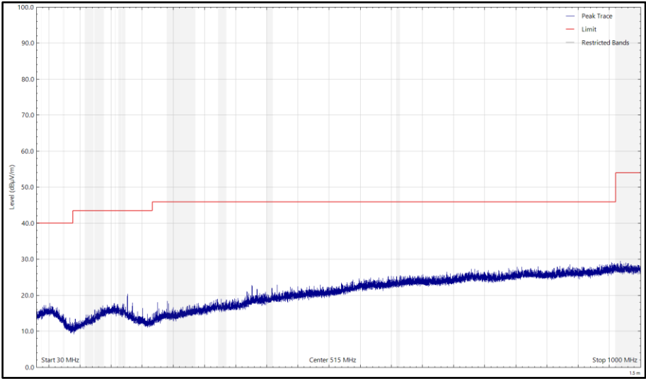
Figure 40 - CH17_LE2M_Z, 2440 MHz, 30 MHz to 1 GHz, Horizontal (Peak)
