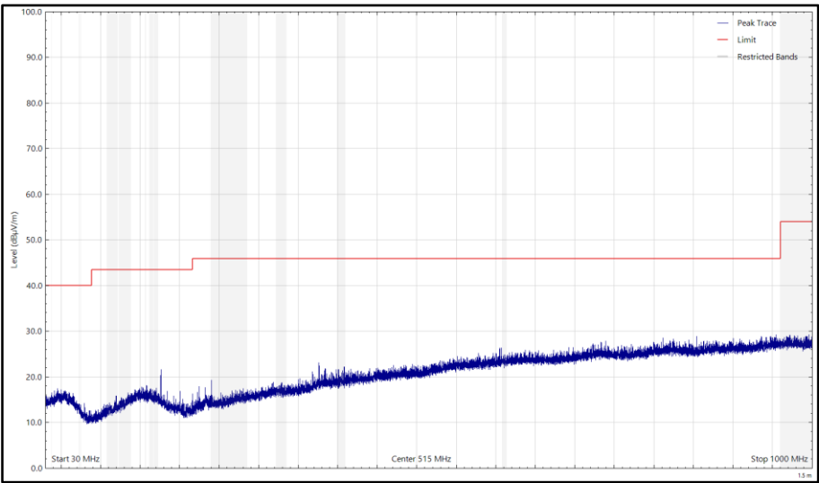
Figure 20 - CH37_LE2M_X, 2404 MHz, 30 MHz to 1 GHz, Horizontal (Peak)
