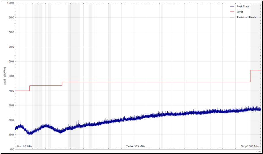
Figure 28 - CH37_LE2M_Z, 2404 MHz, 30 MHz to 1 GHz, Horizontal (Peak)
