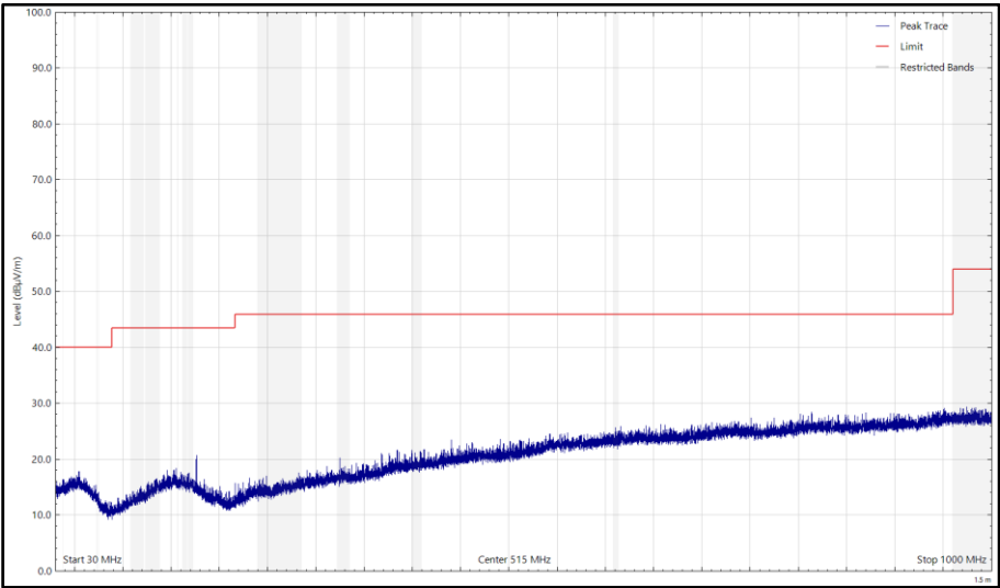
Figure 30 - CH37_LE2M_Z, 2404 MHz, 30 MHz to 1 GHz, Vertical (Peak)
