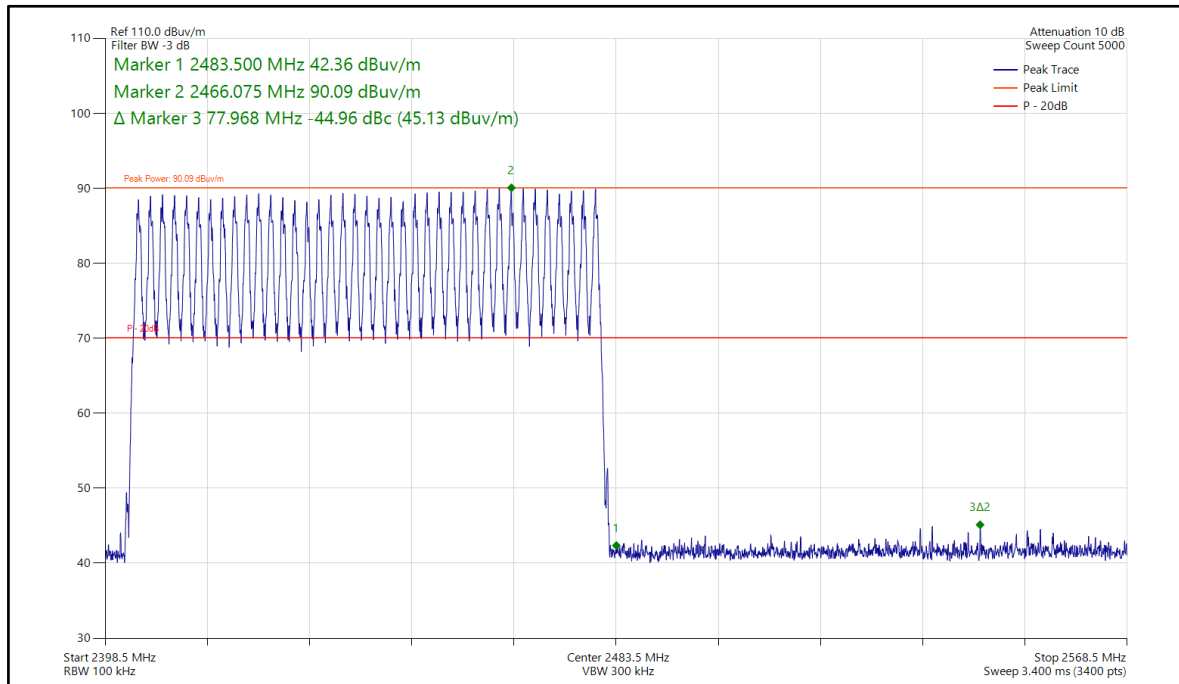
Figure 8 - TOP_FHSS_ABE, 2404-2480 MHz, Band Edge Frequency 2483.5 MHz
