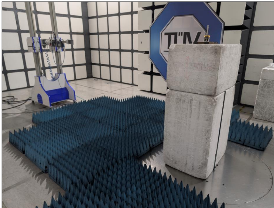
Figure 58 - Test Setup - 8 GHz to 18 GHz
