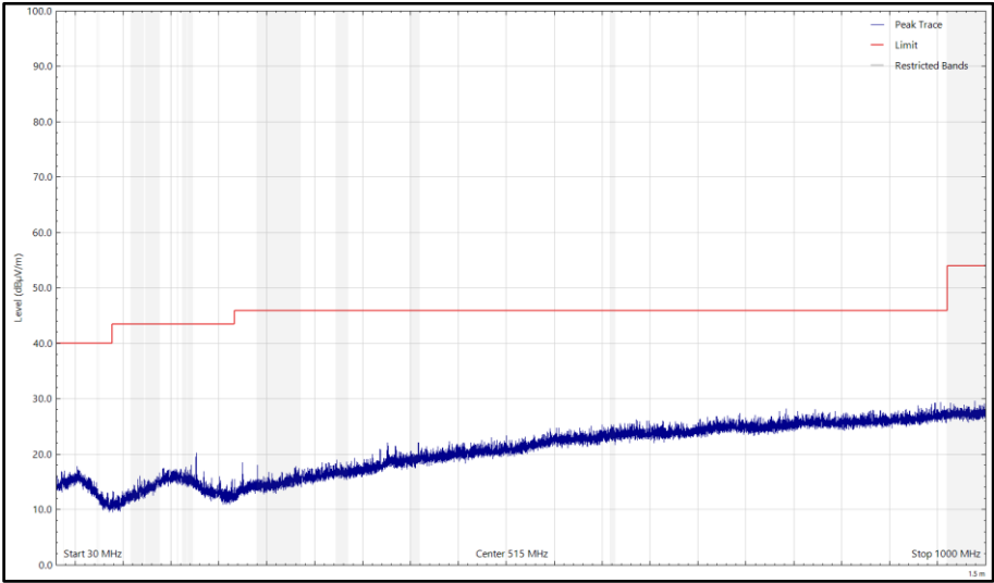
Figure 32 - CH17_LE2M_X, 2440 MHz, 30 MHz to 1 GHz, Horizontal (Peak)
