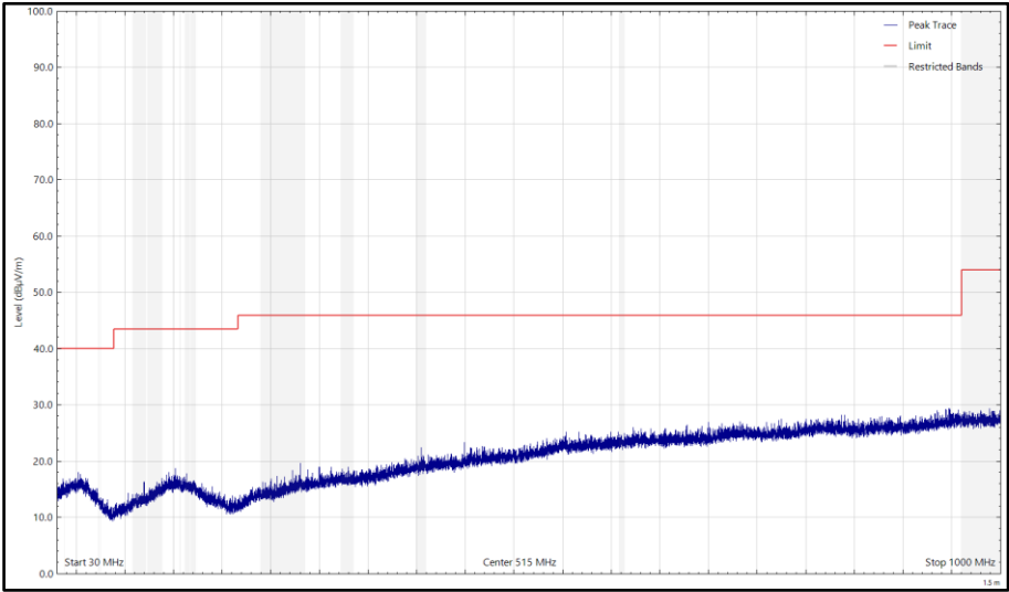
Figure 24 - CH37_LE2M_Y, 2404 MHz, 30 MHz to 1 GHz, Horizontal (Peak)
