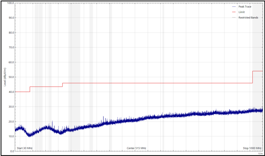
Figure 36 - CH17_LE2M_Y, 2440 MHz, 30 MHz to 1 GHz, Horizontal (Peak)
