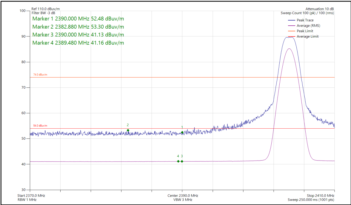
Figure 12 - CH37_BLE2M_RBE, 2404 MHz, Band Edge Frequency 2390 MHz
