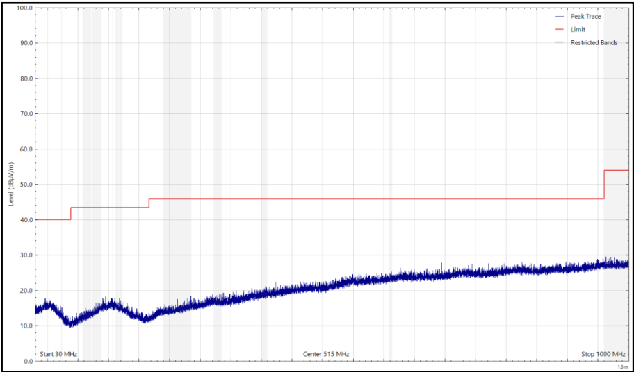
Figure 34 - CH17_LE2M_X, 2440 MHz, 30 MHz to 1 GHz, Vertical (Peak)
