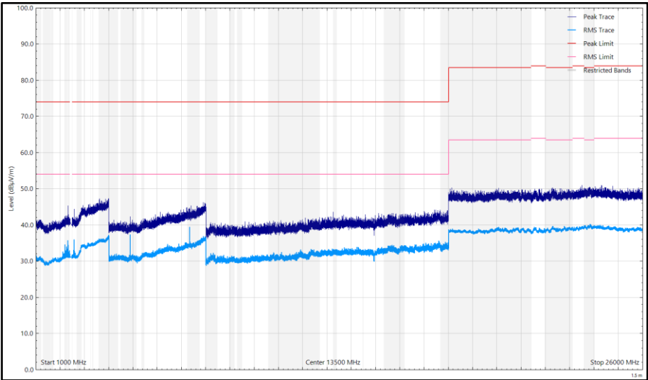
Figure 43 - CH17_LE2M_Z, 2440 MHz, 1 GHz to 26 GHz, Vertical
