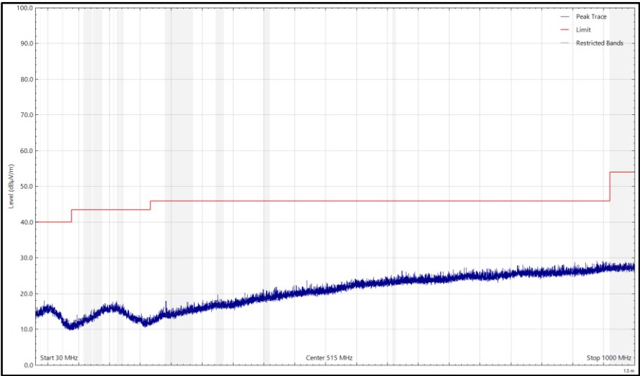
Figure 42 - CH17_LE2M_Z, 2440 MHz, 30 MHz to 1 GHz, Vertical (Peak)
