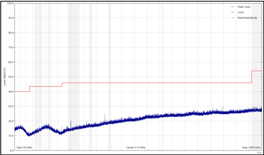
Figure 22 - CH37_LE2M_X, 2404 MHz, 30 MHz to 1 GHz, Vertical (Peak)
