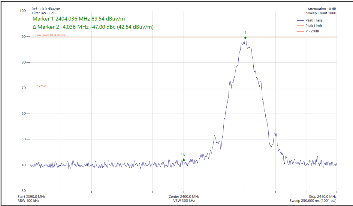
Figure 10 - CH37_BLE2M_ABE, 2404 MHz, Band Edge Frequency 2400 MHz
