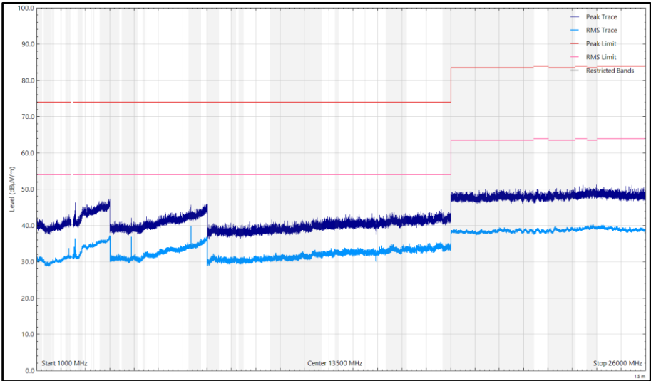
Figure 33 - CH17_LE2M_X, 2440 MHz, 1 GHz to 26 GHz, Horizontal
