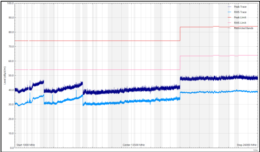
Figure 41 - CH17_LE2M_Z, 2440 MHz, 1 GHz to 26 GHz, Horizontal
