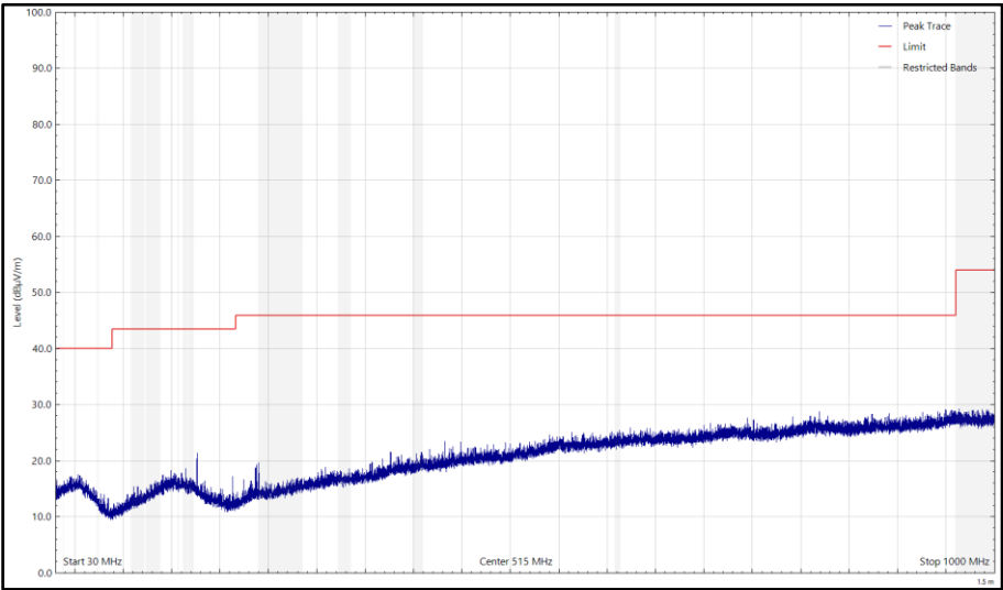
Figure 26 - CH37_LE2M_Y, 2404 MHz, 30 MHz to 1 GHz, Vertical (Peak)
