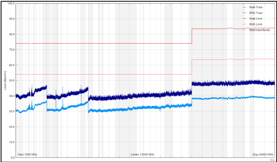
Figure 39 - CH17_LE2M_Y, 2440 MHz, 1 GHz to 26 GHz, Vertical
