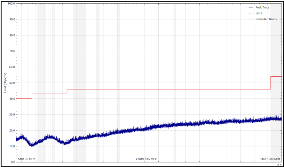
Figure 38 - CH17_LE2M_Y, 2440 MHz, 30 MHz to 1 GHz, Vertical (Peak)
