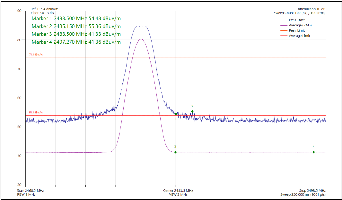
Figure 11 - CH39_BLE2M_RBE, 2480 MHz, Band Edge Frequency 2483.5 MHz
