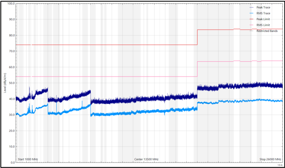
Figure 21 - CH37_LE2M_X, 2404 MHz, 1 GHz to 26 GHz, Horizontal
