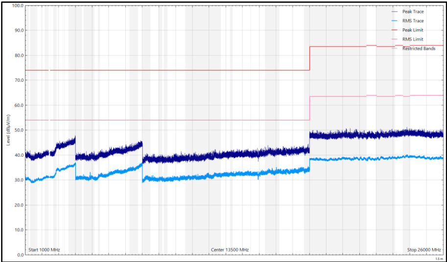
Figure 37 - CH17_LE2M_Y, 2440 MHz, 1 GHz to 26 GHz, Horizontal
