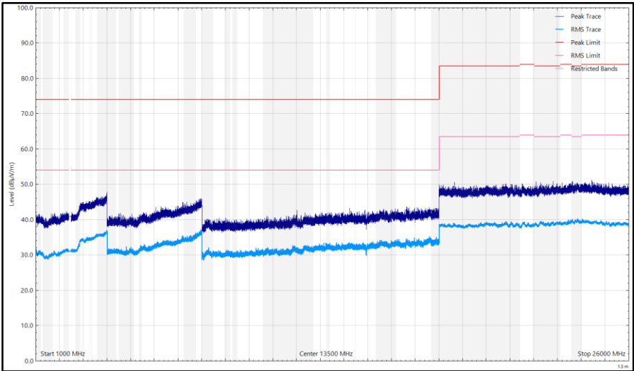
Figure 25 - CH37_LE2M_Y, 2404 MHz, 1 GHz to 26 GHz, Horizontal
