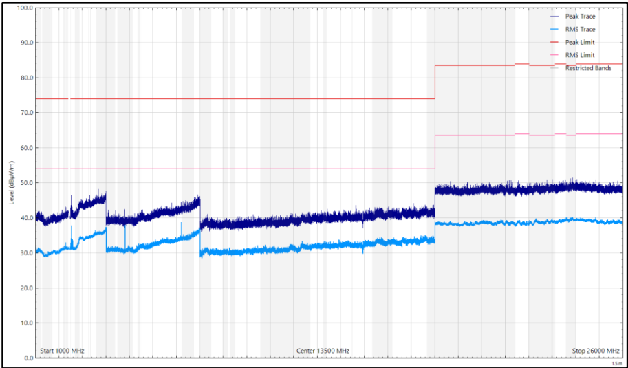
Figure 29 - CH37_LE2M_Z, 2404 MHz, 1 GHz to 26 GHz, Horizontal
