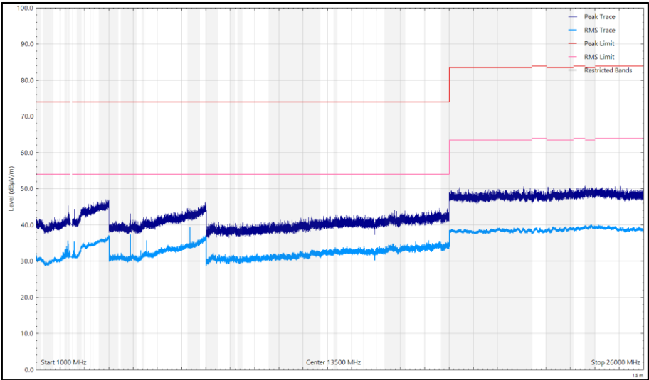
Figure 35 - CH17_LE2M_X, 2440 MHz, 1 GHz to 26 GHz, Vertical
