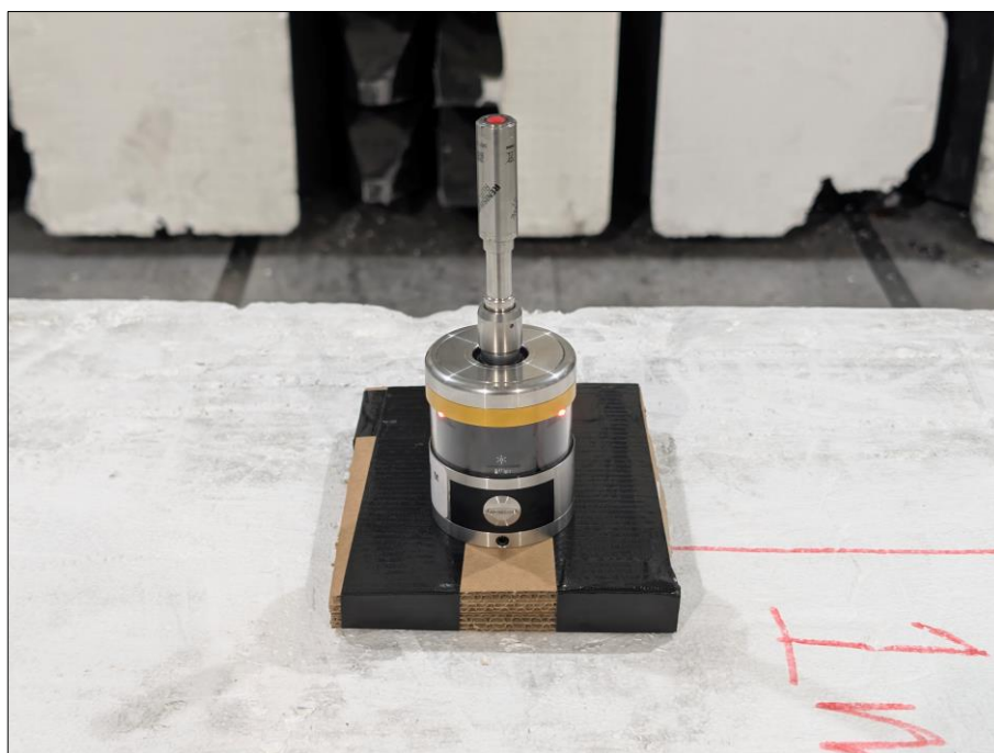
Figure 61 - Test Setup – Y Orientation
