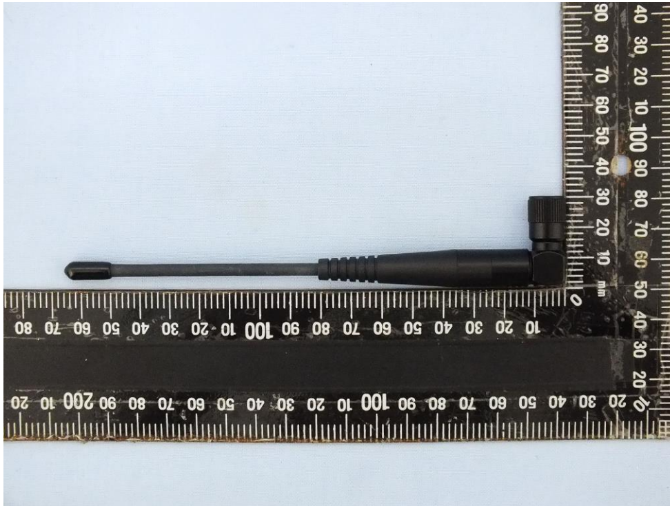
Antenna model: S161AH-915R
