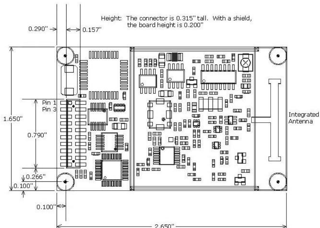
Figure 1. Mechanical Overview of LX2400S
