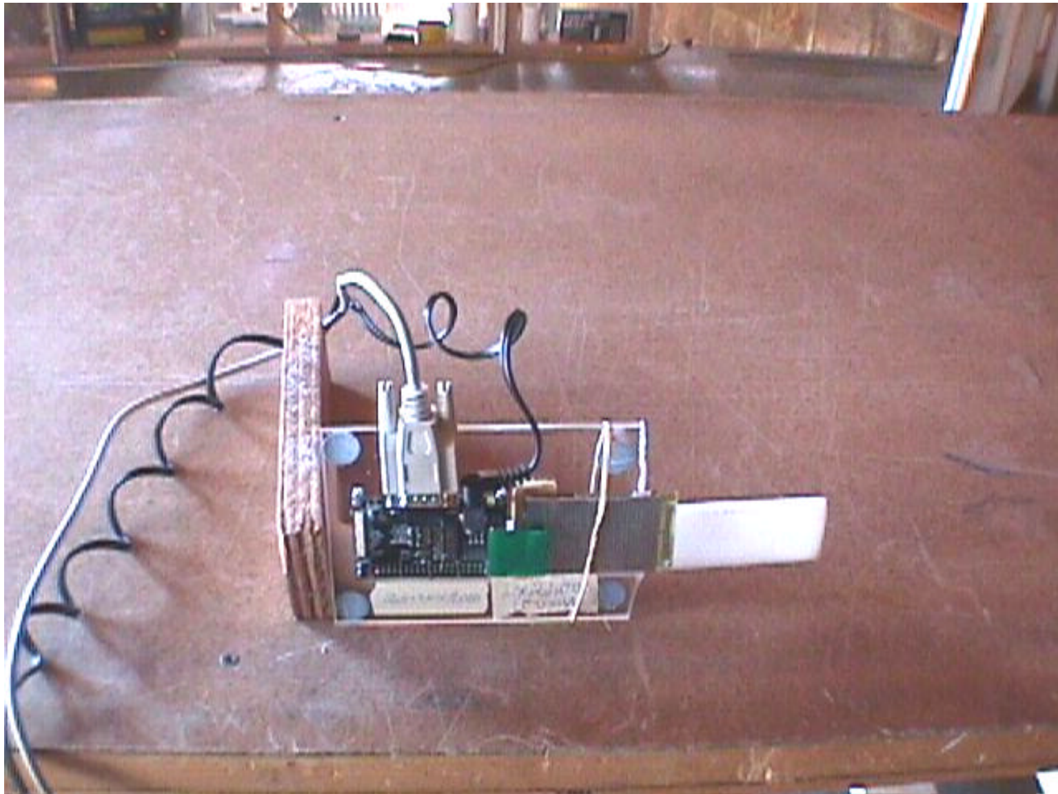
Exhibit 10 - Setup Photographs Aerocomm LX2400-3 with Aerocomm NZH2400-I Antenna
