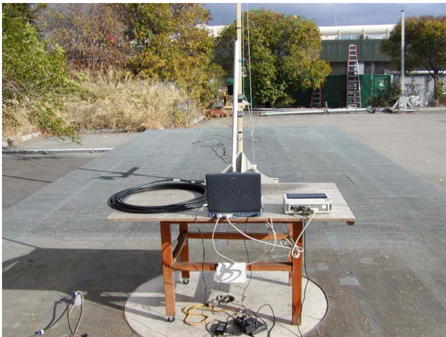
Radiated Emission with MFB24012 Antenna - Rear View
