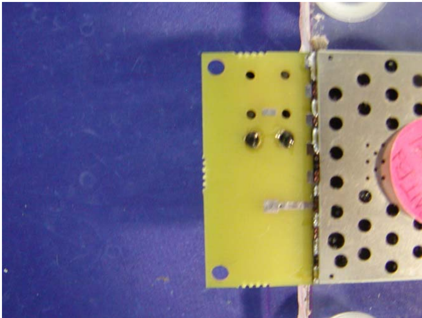
Flavus 915MHz Antenna – Top View
