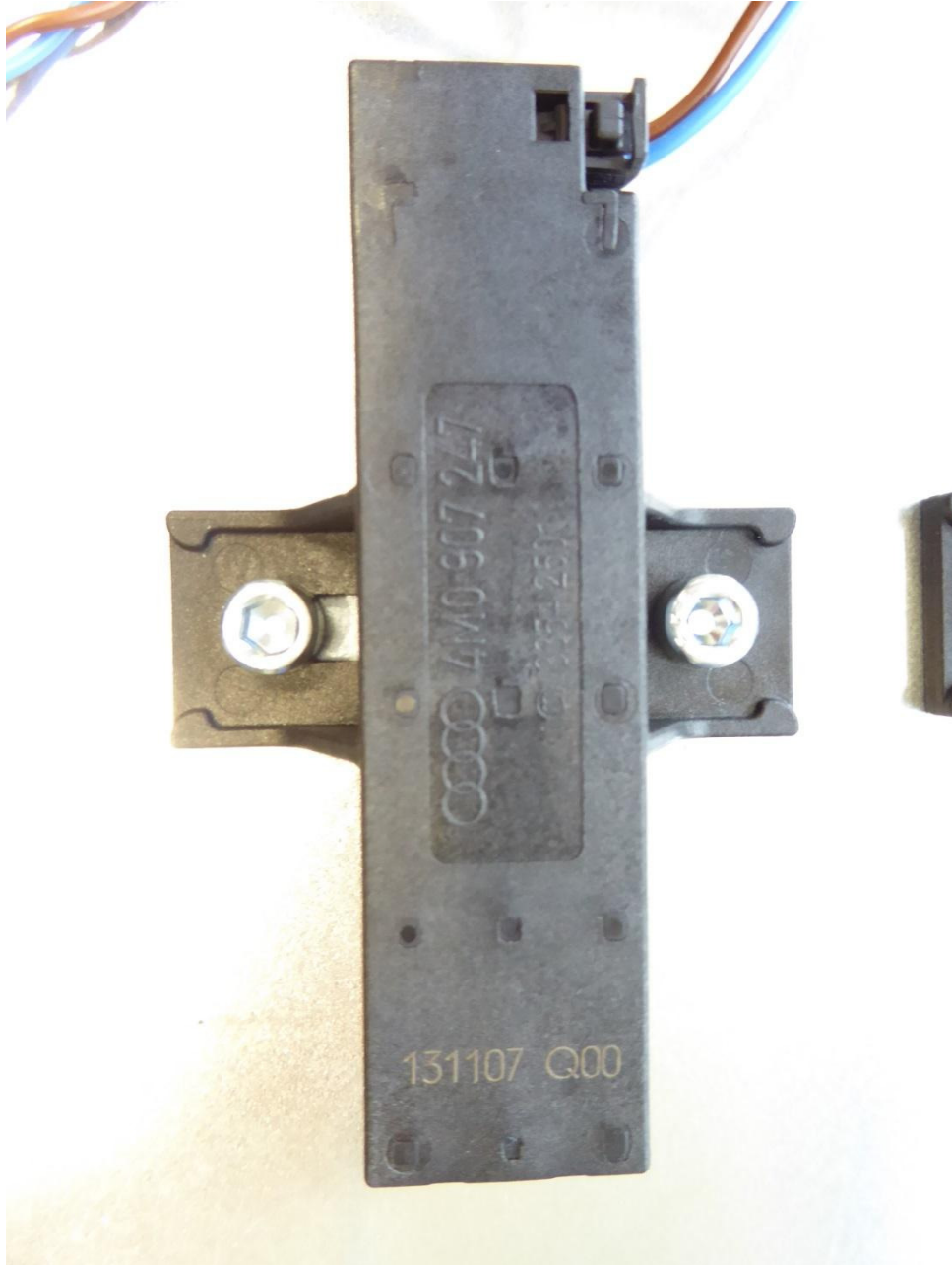
154295_8.JPG: LF antenna type 1
