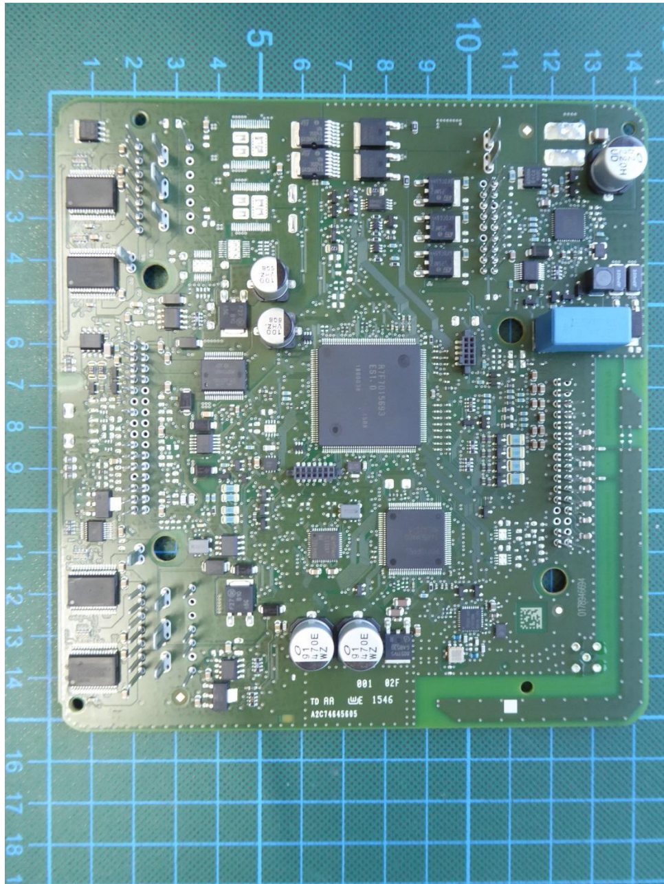
154295_7.JPG: EUT, PCB, bottom view
