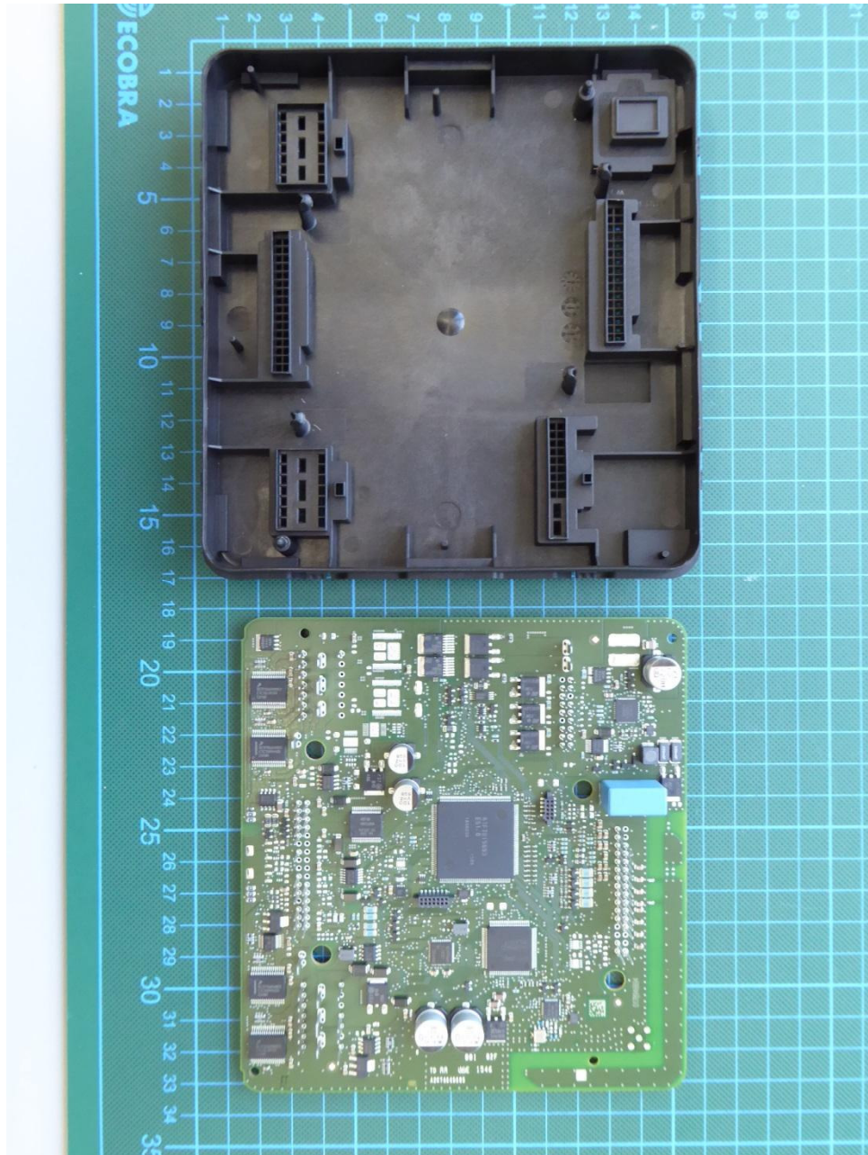
154295_6.JPG: EUT, PCB bottom view, bottom cover removed
