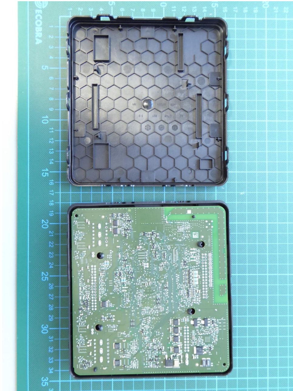
154295_4.JPG: EUT, PCB, top view, top cover removed
