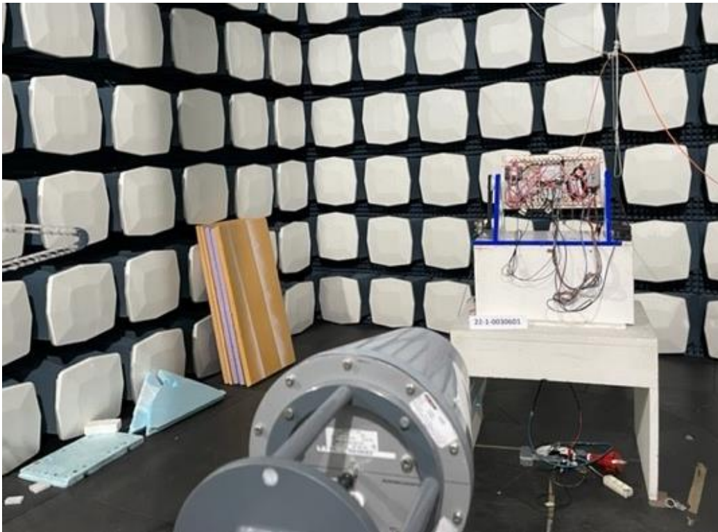
Fig. Mea.: 3 : Radiated RF Parameter > 1GHz Image overview, FAC 1
