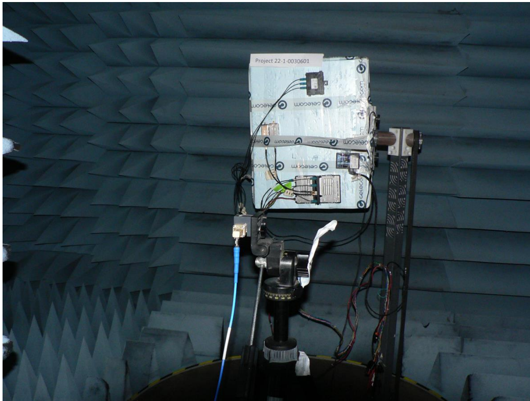
Fig. Mea.: 5 : Radiated RF Parameter > 15GHz Image overview, FAC 2
