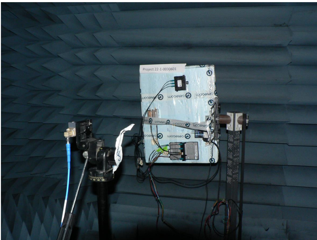
Fig. Mea.: 4 : Radiated RF Parameter > 15GHz Image close up view, FAC 2
