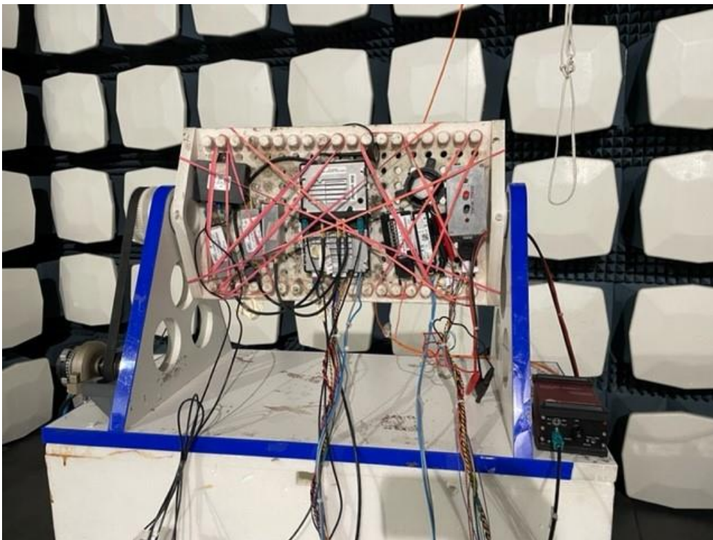
Fig. Mea.: 2 : Radiated RF Parameter > 1GHz Image close up view, FAC 1
