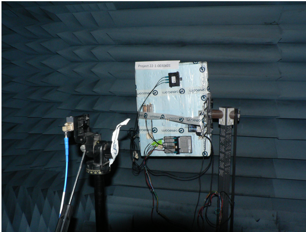
Fig. Mea.: 3 : Radiated RF Parameter Image close up view, FAC 2
