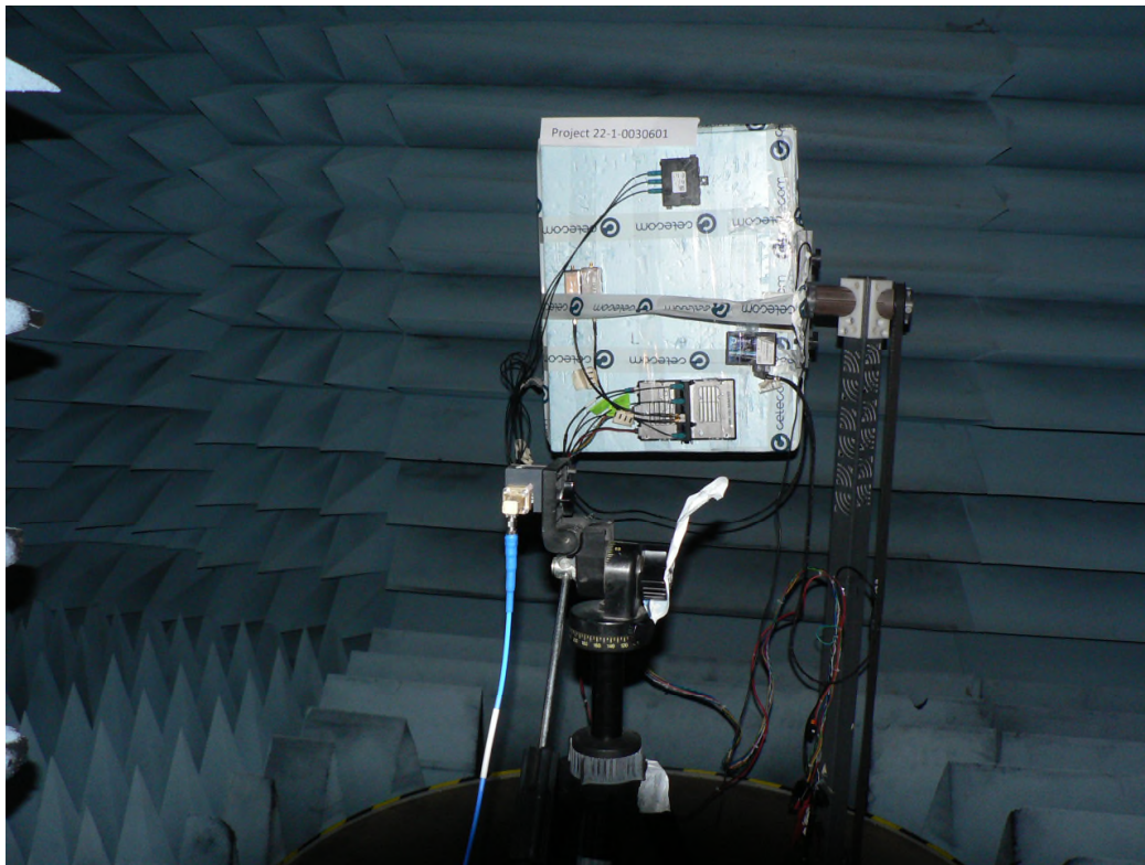
Fig. Mea.: 4 : Radiated RF Parameter Image overview, FAC 2
