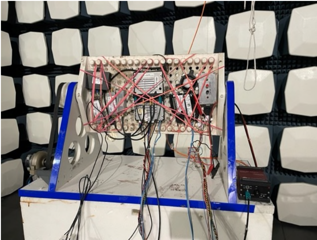
Fig. Mea.: 1 : Radiated RF Parameter Image close up view, FAC 1
