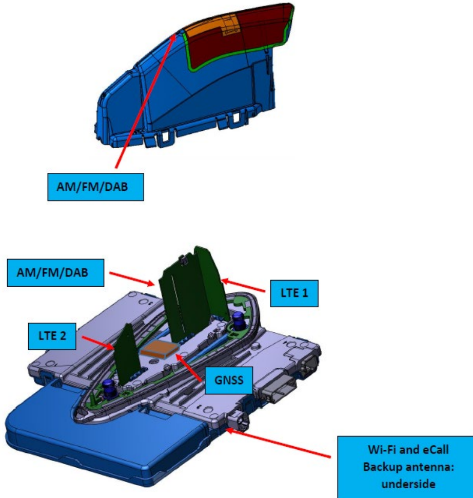
Figure 3: The location of the antennas
