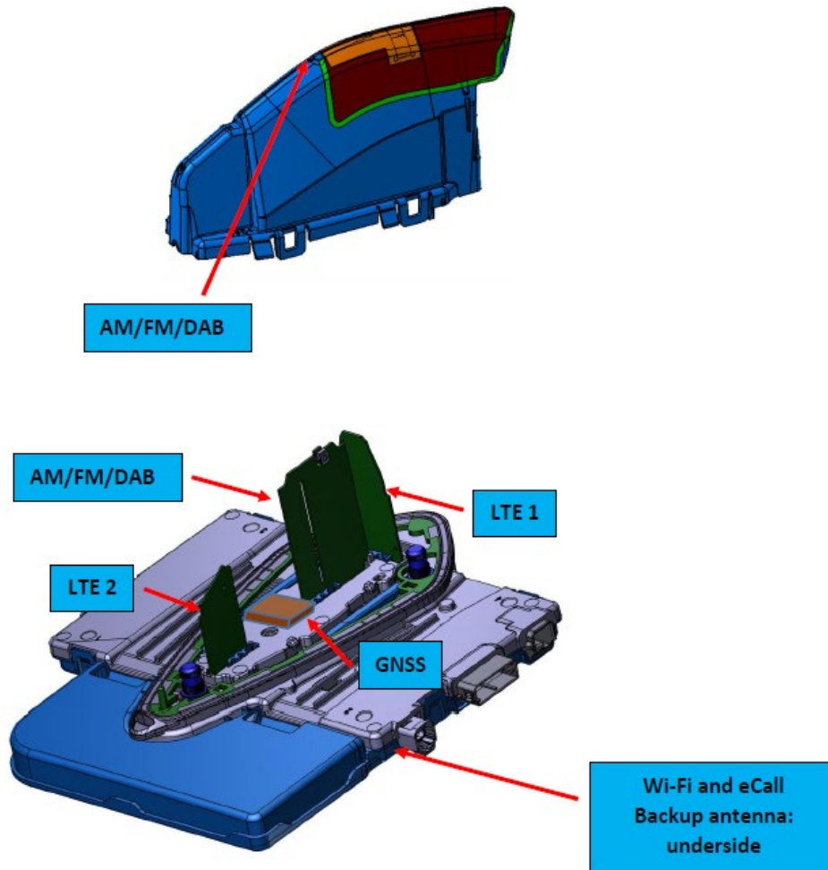
Figure 2: The location of the antennas
