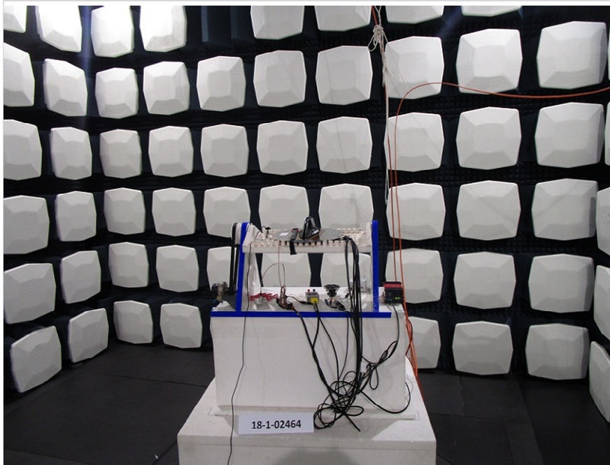
Photograph 3: EUT test setup in the fully anechoic chamber, close up view
