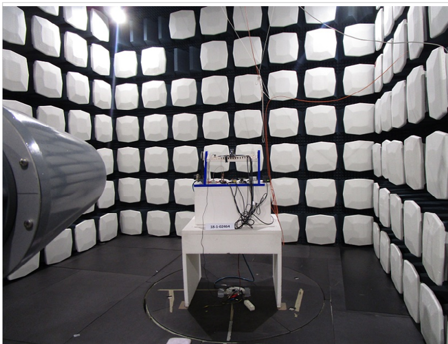
Photograph 4: EUT test setup in the fully anechoic chamber, overview
