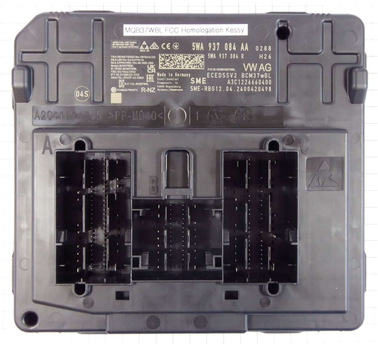
Top view
