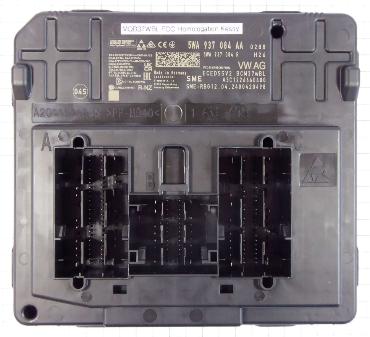
Top view
