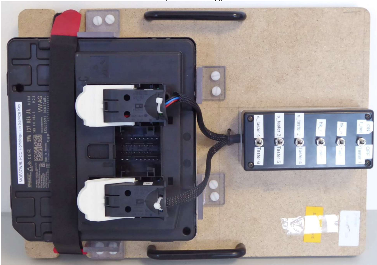
Top view – Test jig
