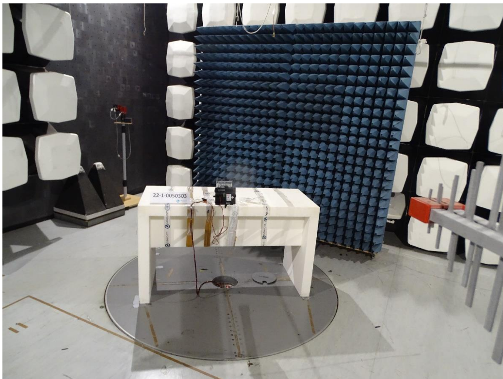
Photograph 2 : Radiated Emission setup picture
