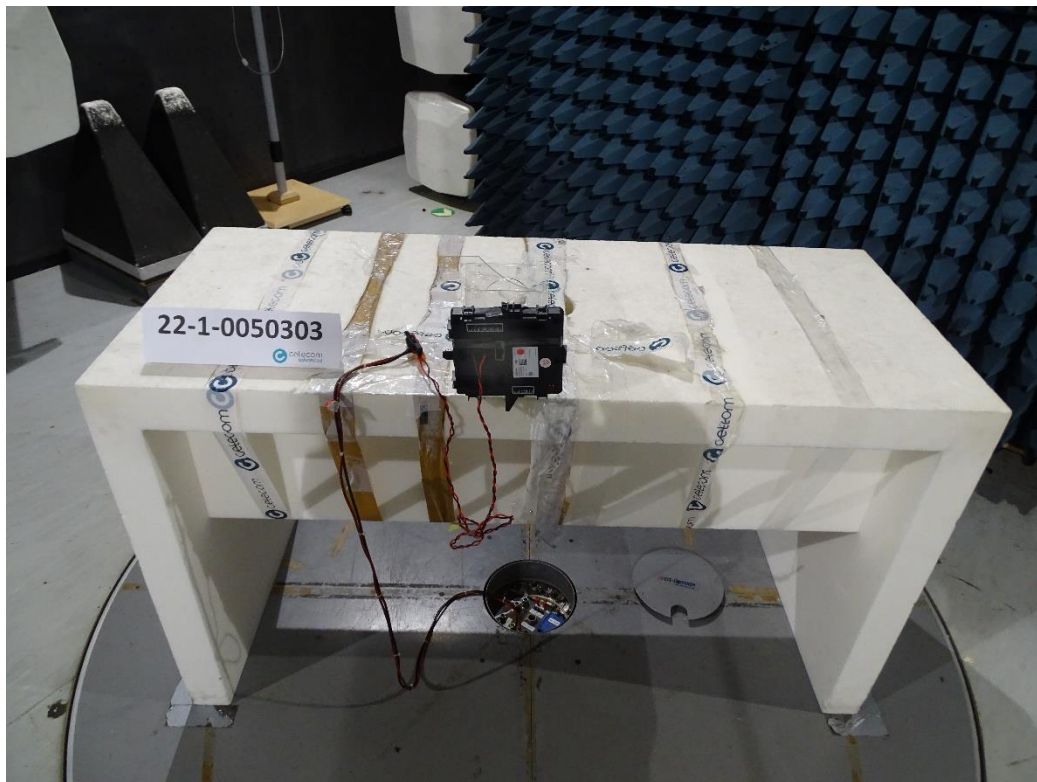
Photograph 1 : Radiated Emission Radiated setup picture
