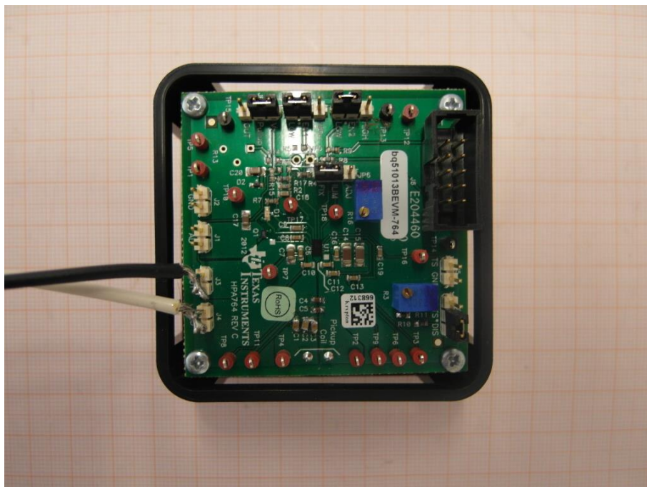
Photo 10 (wireless dummy load unit front view):
