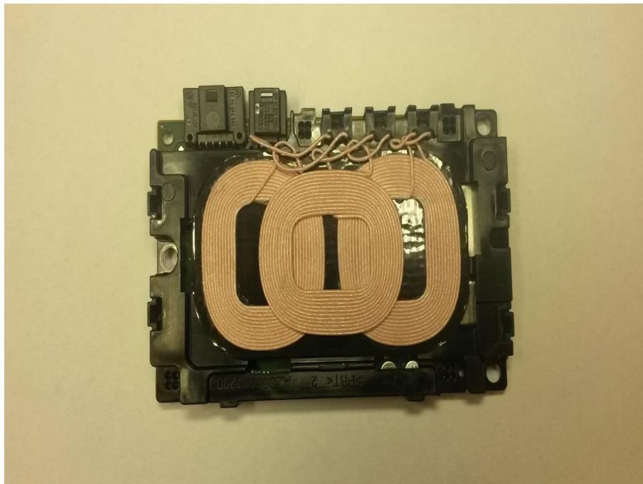
Photo 5 (EUT internal antennas):
