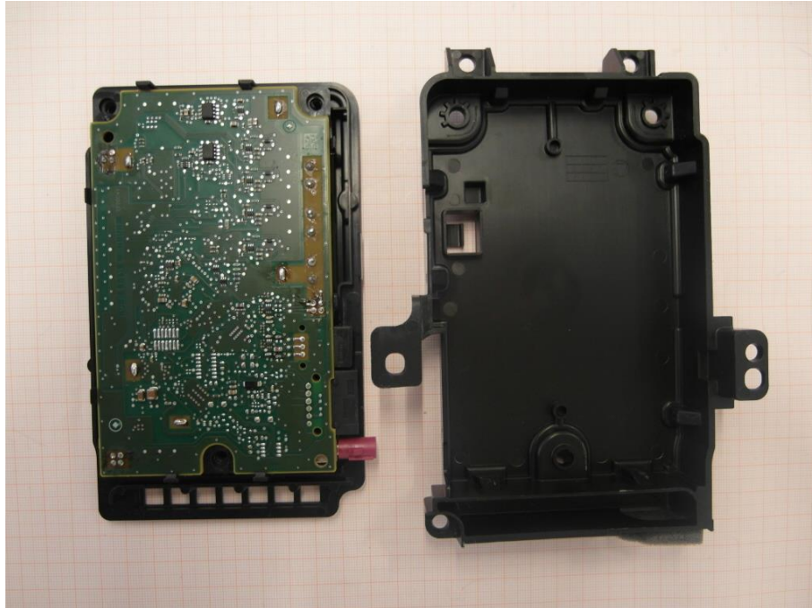
Photo 1 (EUT unmounted case front view):
