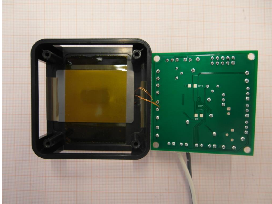
Photo 9 (wireless dummy load unit inner view):
