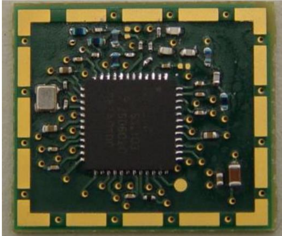
Photo No. 16: HF module without shielding (provided by applicant)
