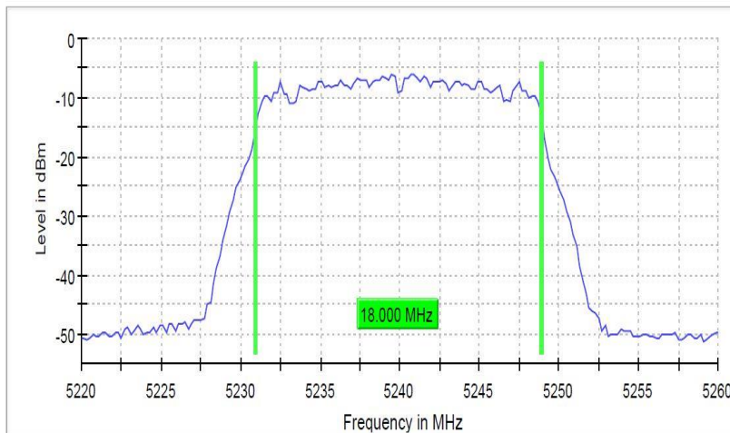
99 % Bandwidth
