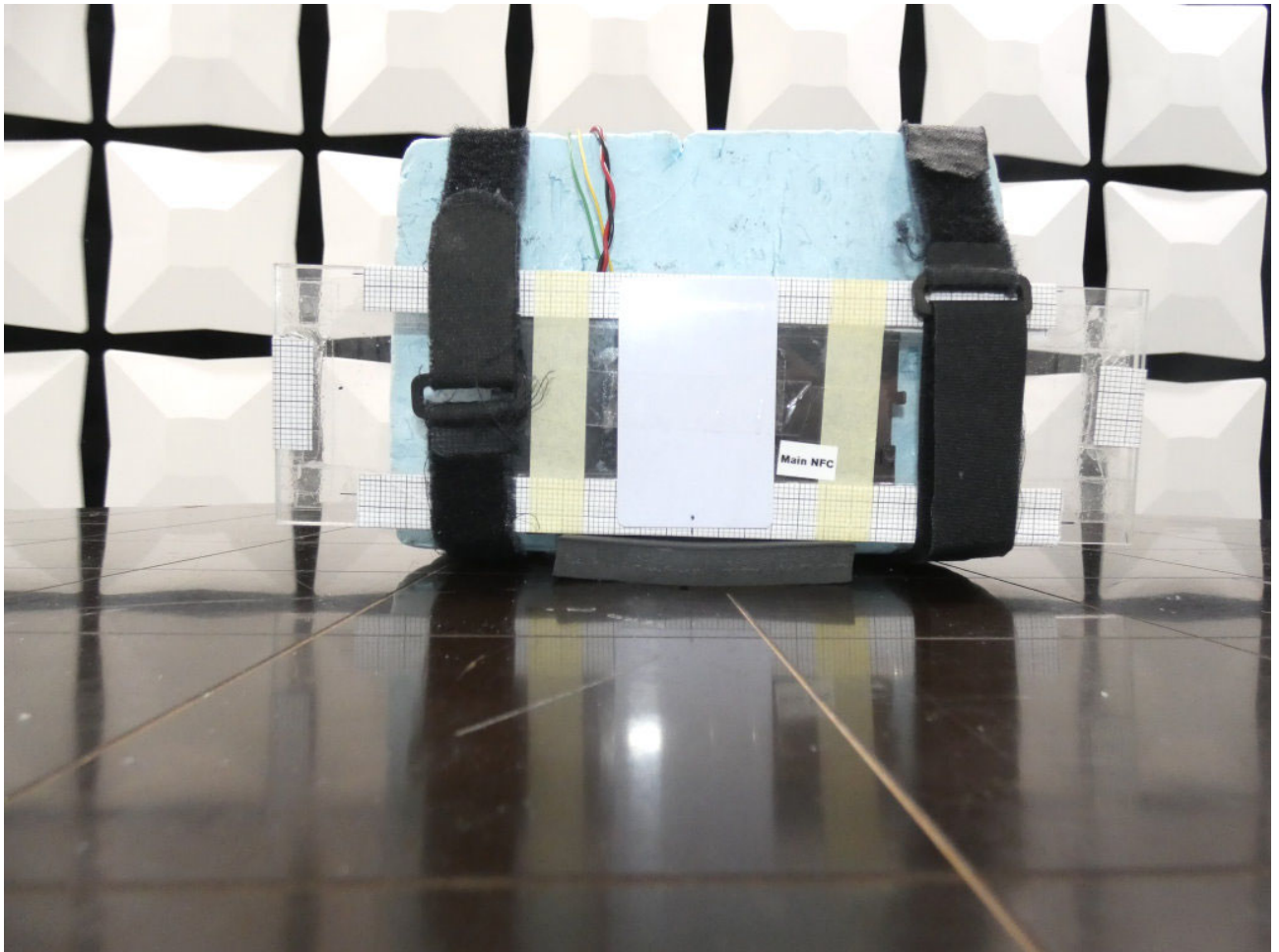
Photo 3: Test setup of EUT in vertical position, central (main) antenna, intentional radiator §15, ANSI C63.10
