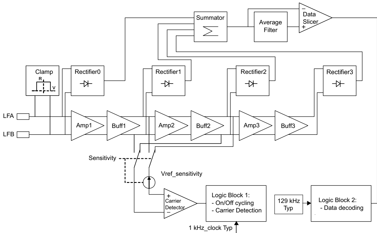
Figure 65. Block Diagram
