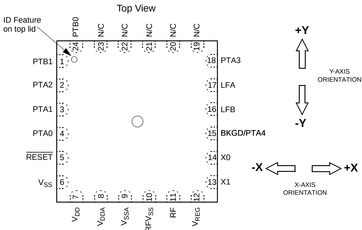
Figure 3. FXTH870x6 QFN Package Pinout
