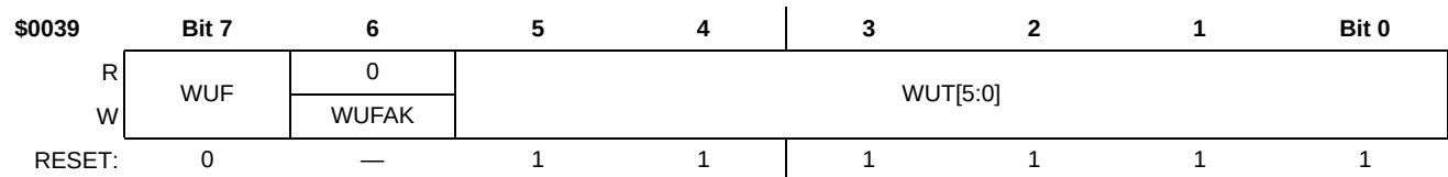
Figure 62. PWU Control/Status Register 0 (PWUCS0)
