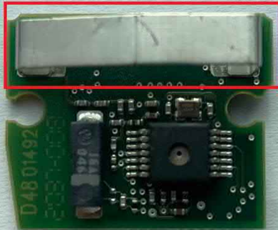
UHF antenna
