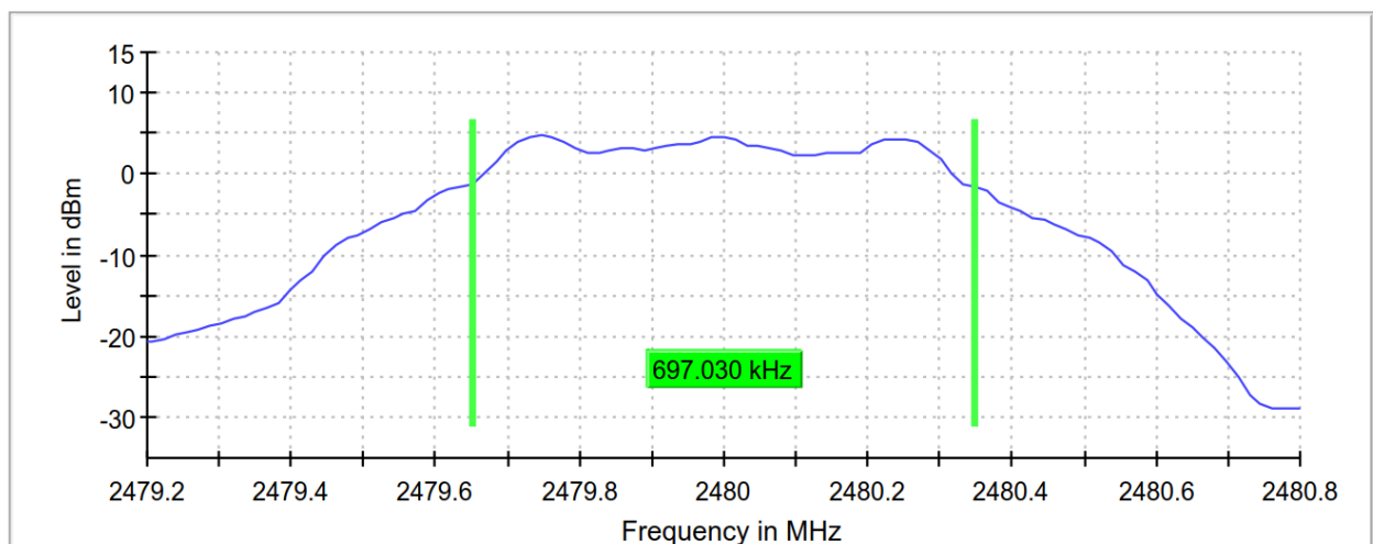
6 dB Bandwidth
