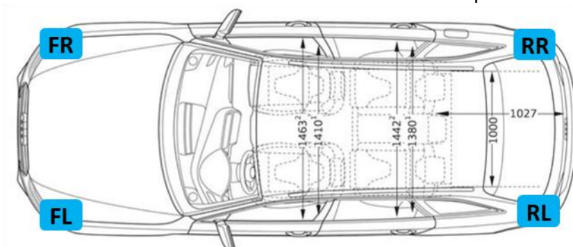
Example schematic
