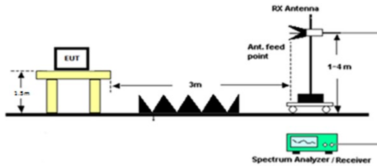
Drawing of Radiated Emissions Test Setup Above 1000 MHz
