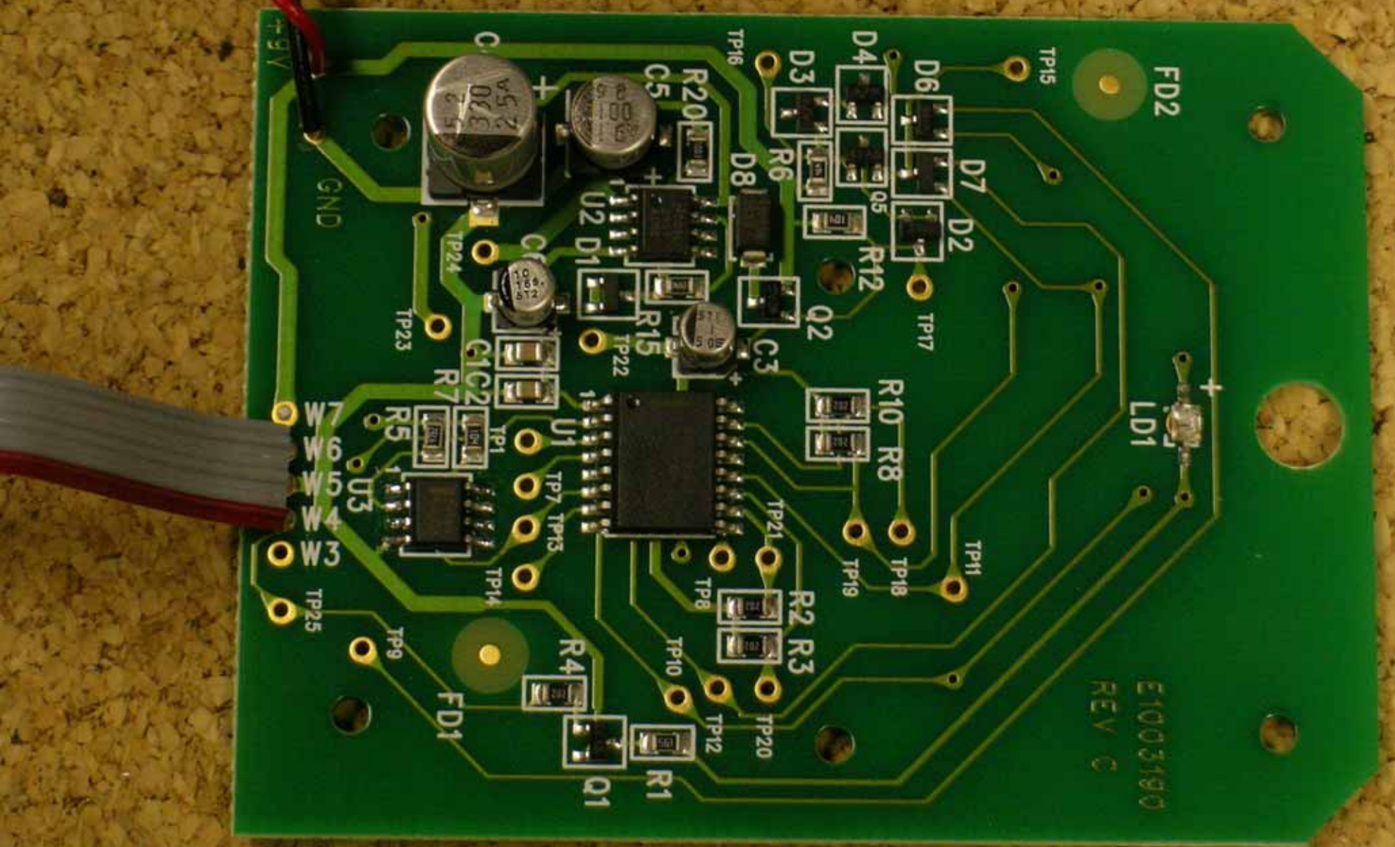
PCB (bottom)
