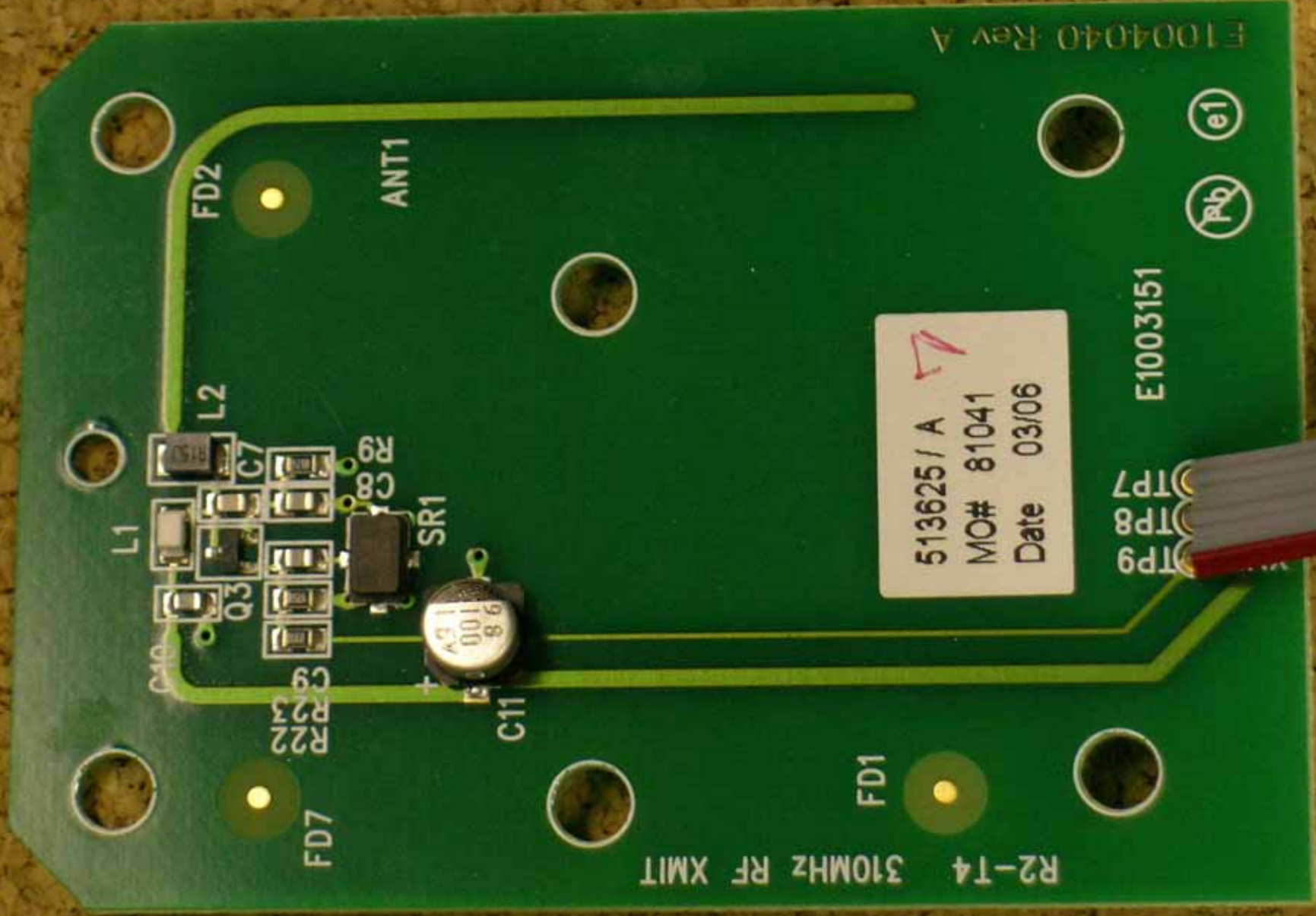
PCB (top)
